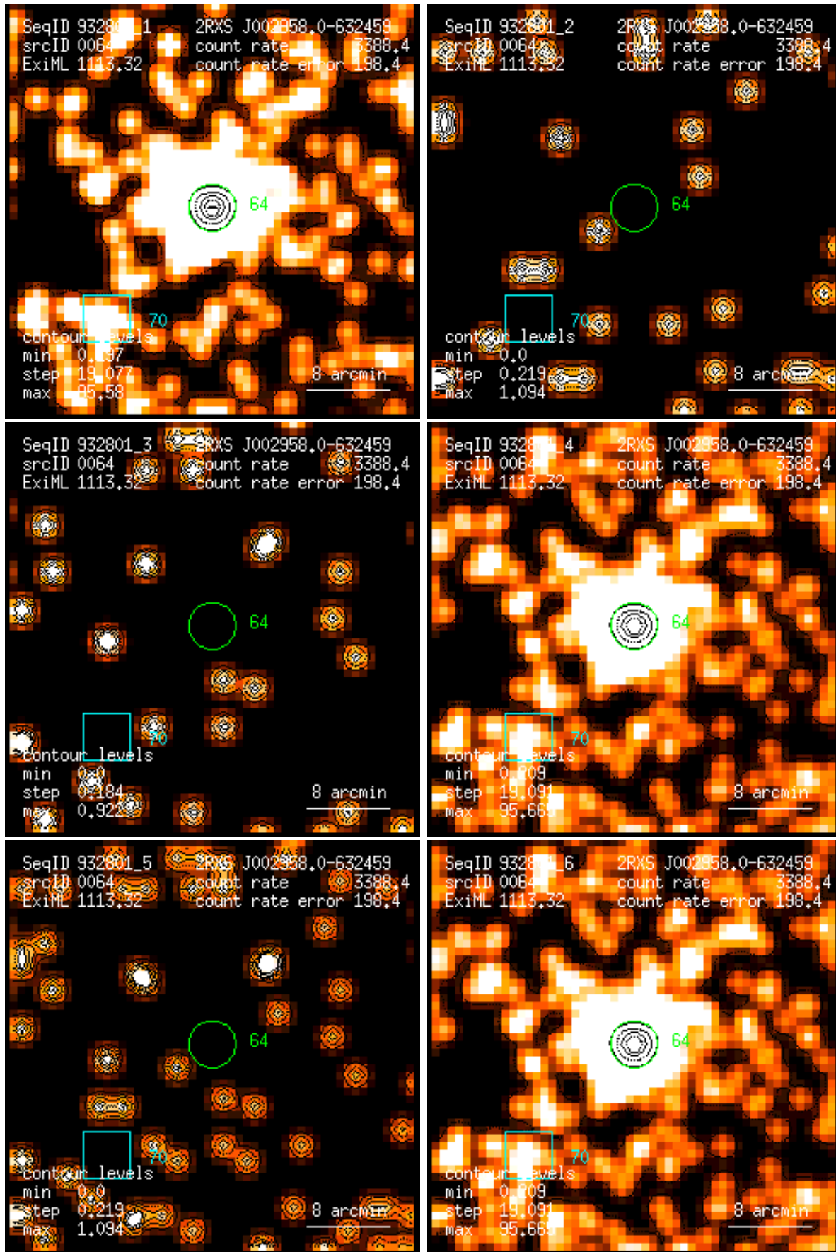
Figure 64: RASS 932801: detection 0064: band rate images, Gaussian filter: (1) PSPC channels 11 – 41, (2) 52 – 90, (3) 91 – 201, (4) 11 – 235, (5) 52 – 201, (6) 11 – 201. Broad band rates in counts/ks. Band rate contour levels in counts/ks/arcmin 2 .
