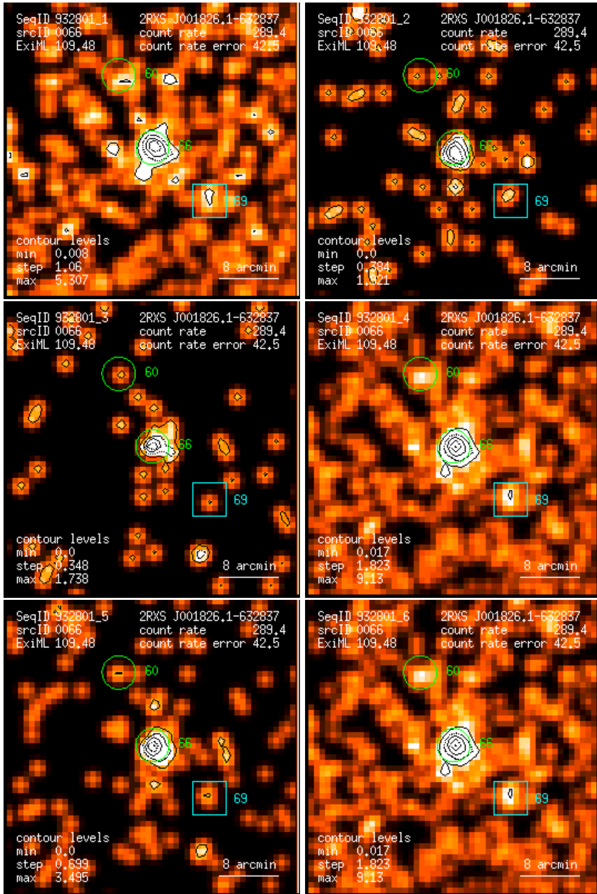
Figure 66: RASS 932801: detection 0066: band rate images, Gaussian filter: (1) PSPC channels 11 – 41, (2) 52 – 90, (3) 91 – 201, (4) 11 – 235, (5) 52 – 201, (6) 11 – 201. Broad band rates in counts/ks. Band rate contour levels in counts/ks/arcmin 2 .
