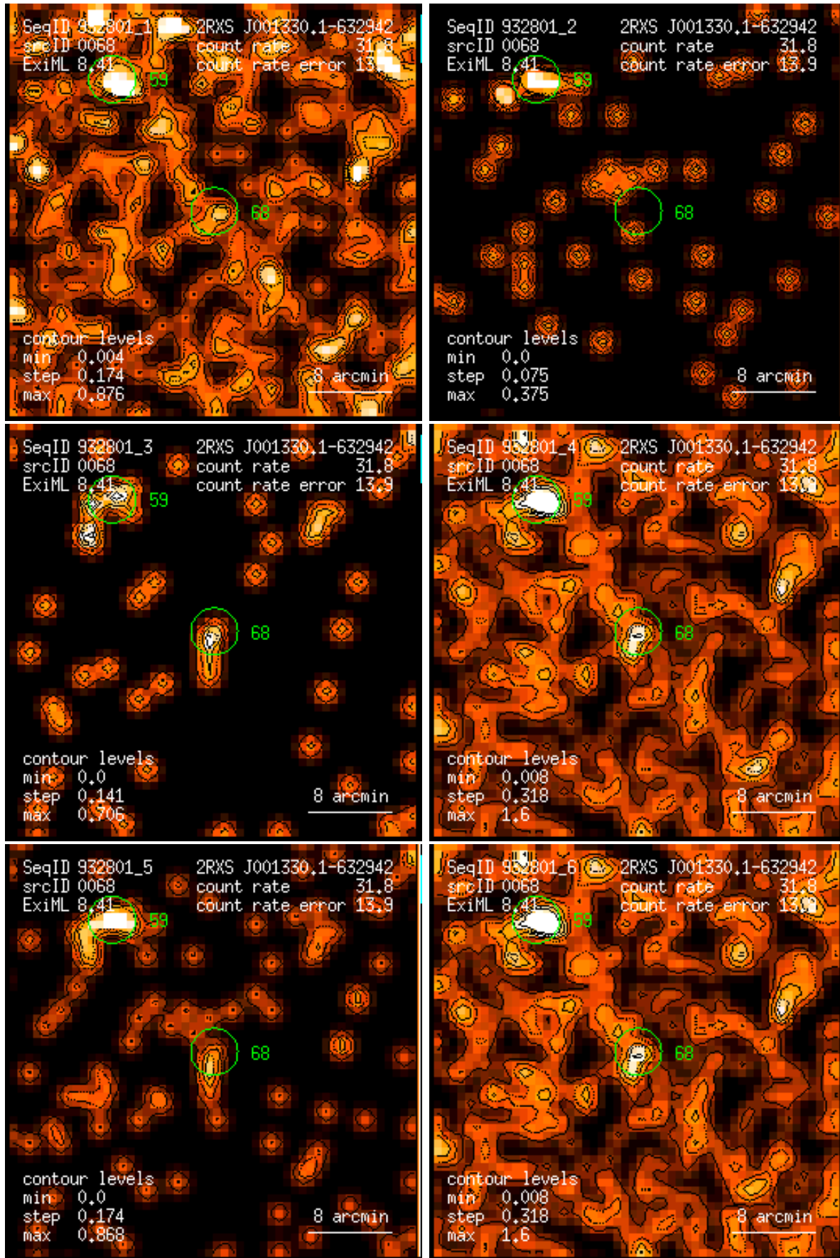
Figure 68: RASS 932801: detection 0068: band rate images, Gaussian filter: (1) PSPC channels 11 – 41, (2) 52 – 90, (3) 91 – 201, (4) 11 – 235, (5) 52 – 201, (6) 11 – 201. Broad band rates in counts/ks. Band rate contour levels in counts/ks/arcmin 2 .
