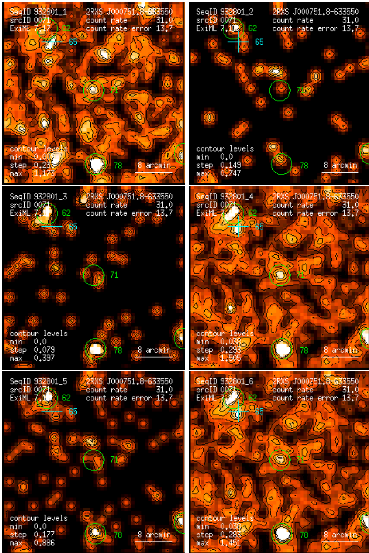
Figure 71: RASS 932801: detection 0071: band rate images, Gaussian filter: (1) PSPC channels 11 – 41, (2) 52 – 90, (3) 91 – 201, (4) 11 – 235, (5) 52 – 201, (6) 11 – 201. Broad band rates in counts/ks. Band rate contour levels in counts/ks/arcmin 2 .
