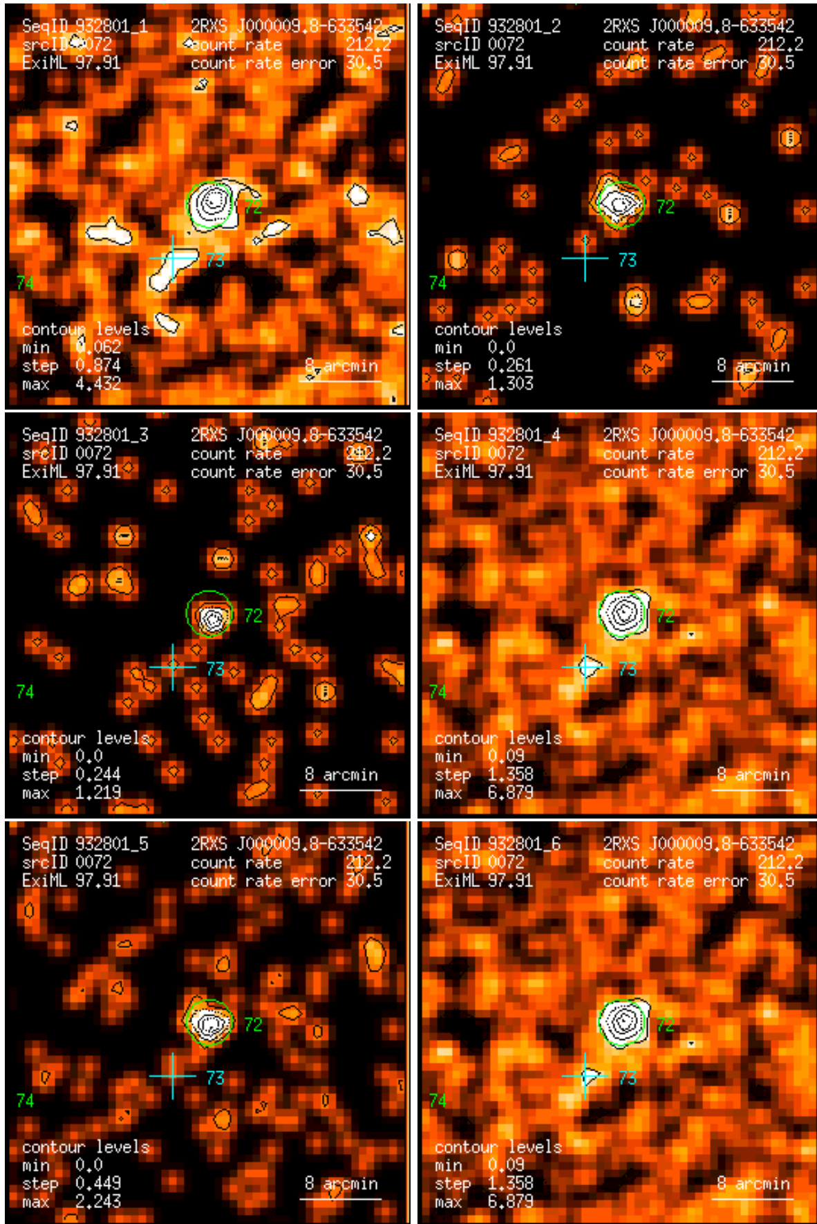
Figure 72: RASS 932801: detection 0072: band rate images, Gaussian filter: (1) PSPC channels 11 – 41, (2) 52 – 90, (3) 91 – 201, (4) 11 – 235, (5) 52 – 201, (6) 11 – 201. Broad band rates in counts/ks. Band rate contour levels in counts/ks/arcmin 2 .
