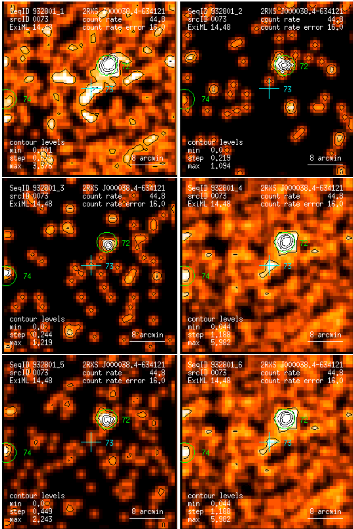
Figure 73: RASS 932801: detection 0073: band rate images, Gaussian filter: (1) PSPC channels 11 – 41, (2) 52 – 90, (3) 91 – 201, (4) 11 – 235, (5) 52 – 201, (6) 11 – 201. Broad band rates in counts/ks. Band rate contour levels in counts/ks/arcmin 2 .
