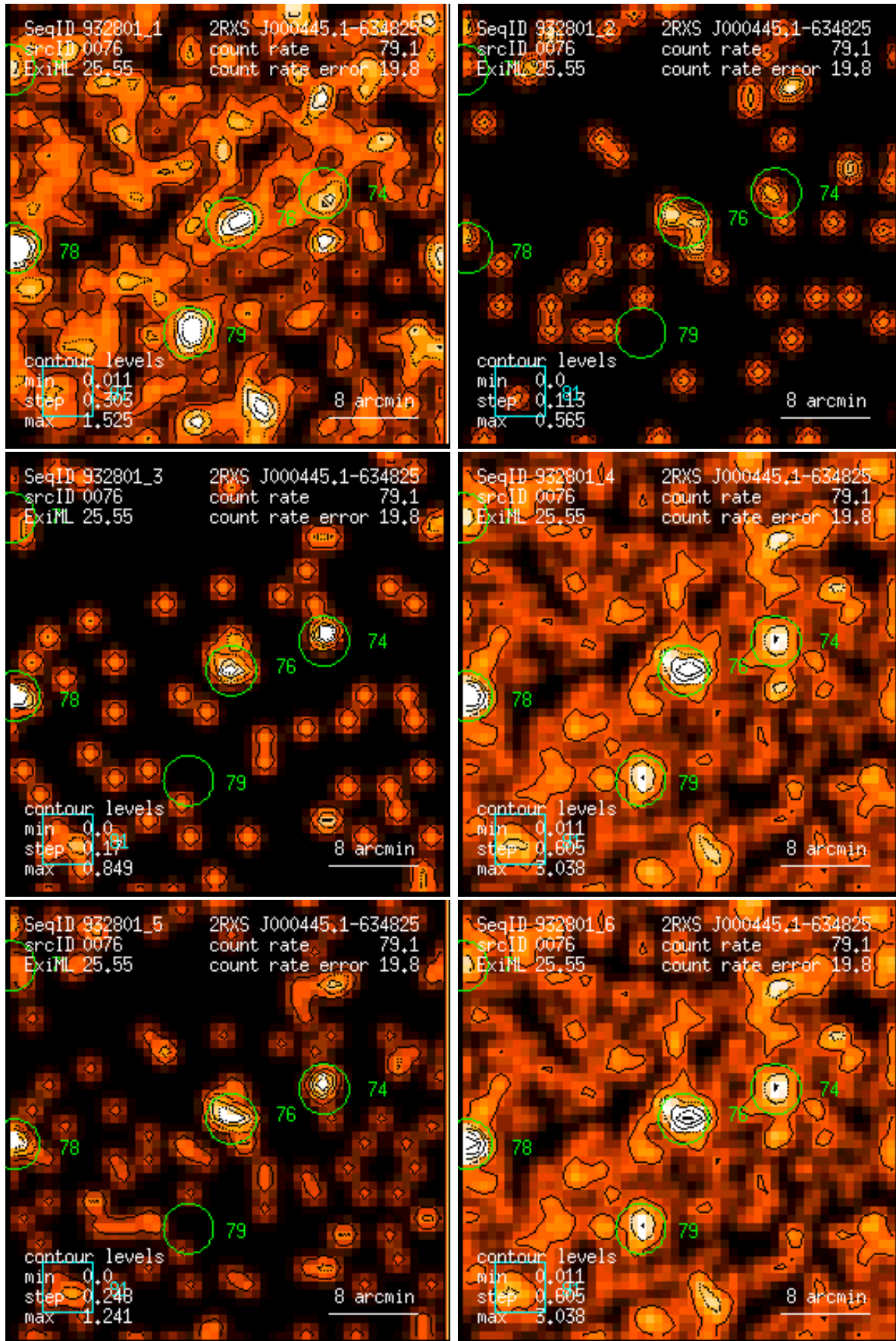
Figure 76: RASS 932801: detection 0076: band rate images, Gaussian filter: (1) PSPC channels 11 – 41, (2) 52 – 90, (3) 91 – 201, (4) 11 – 235, (5) 52 – 201, (6) 11 – 201. Broad band rates in counts/ks. Band rate contour levels in counts/ks/arcmin 2 .
