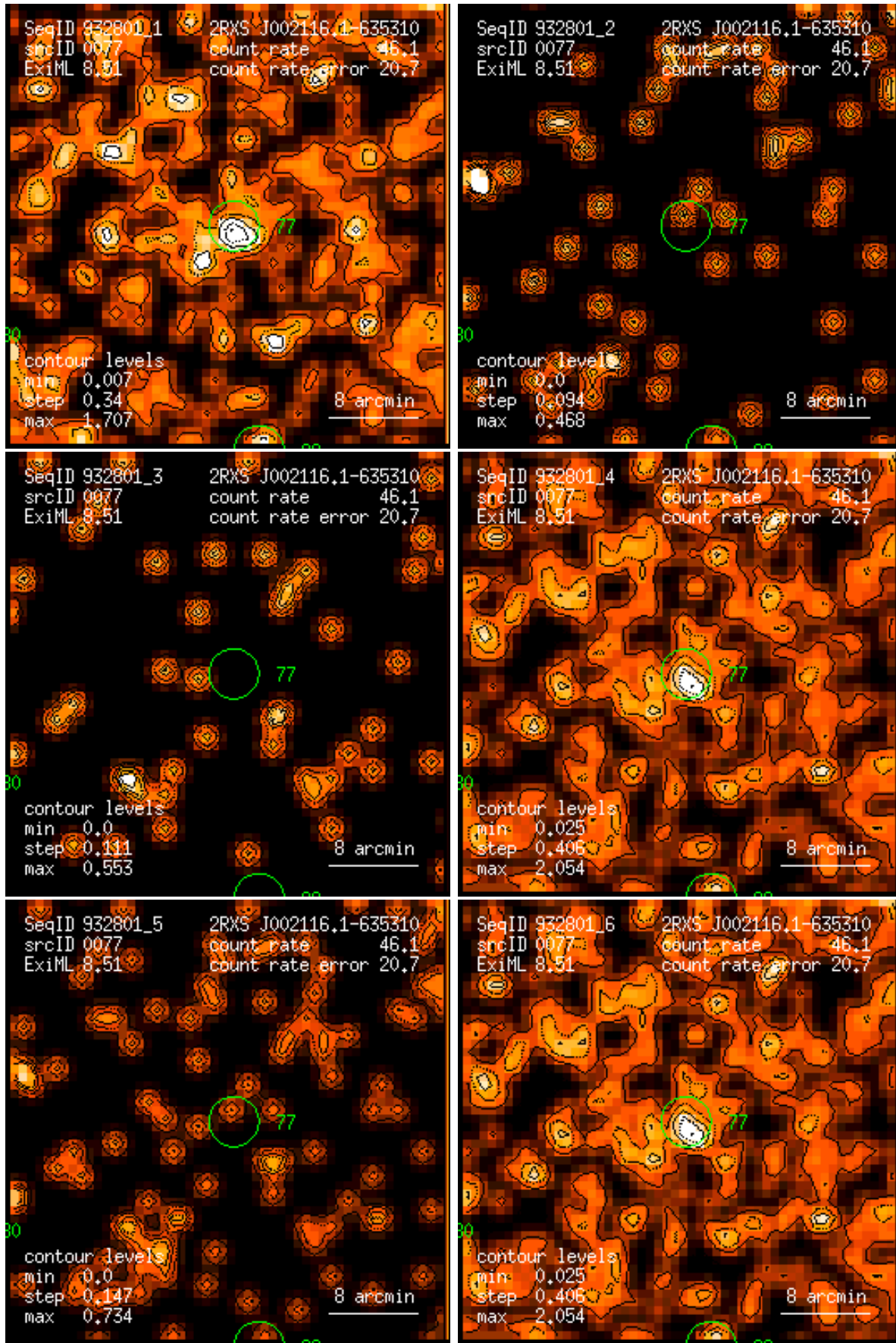
Figure 77: RASS 932801: detection 0077: band rate images, Gaussian filter: (1) PSPC channels 11 – 41, (2) 52 – 90, (3) 91 – 201, (4) 11 – 235, (5) 52 – 201, (6) 11 – 201. Broad band rates in counts/ks. Band rate contour levels in counts/ks/arcmin 2 .
