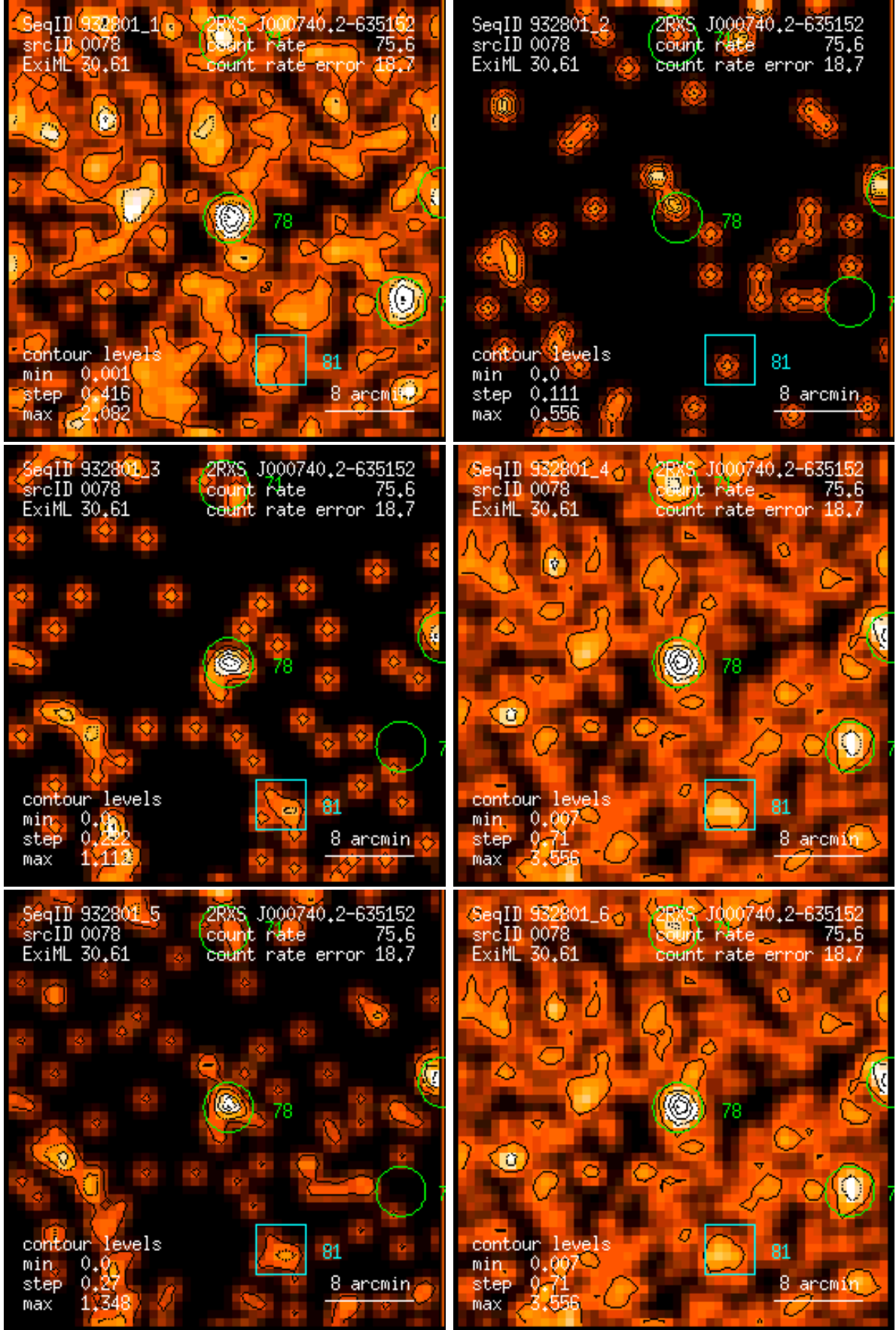
Figure 78: RASS 932801: detection 0078: band rate images, Gaussian filter: (1) PSPC channels 11 – 41, (2) 52 – 90, (3) 91 – 201, (4) 11 – 235, (5) 52 – 201, (6) 11 – 201. Broad band rates in counts/ks. Band rate contour levels in counts/ks/arcmin 2 .
