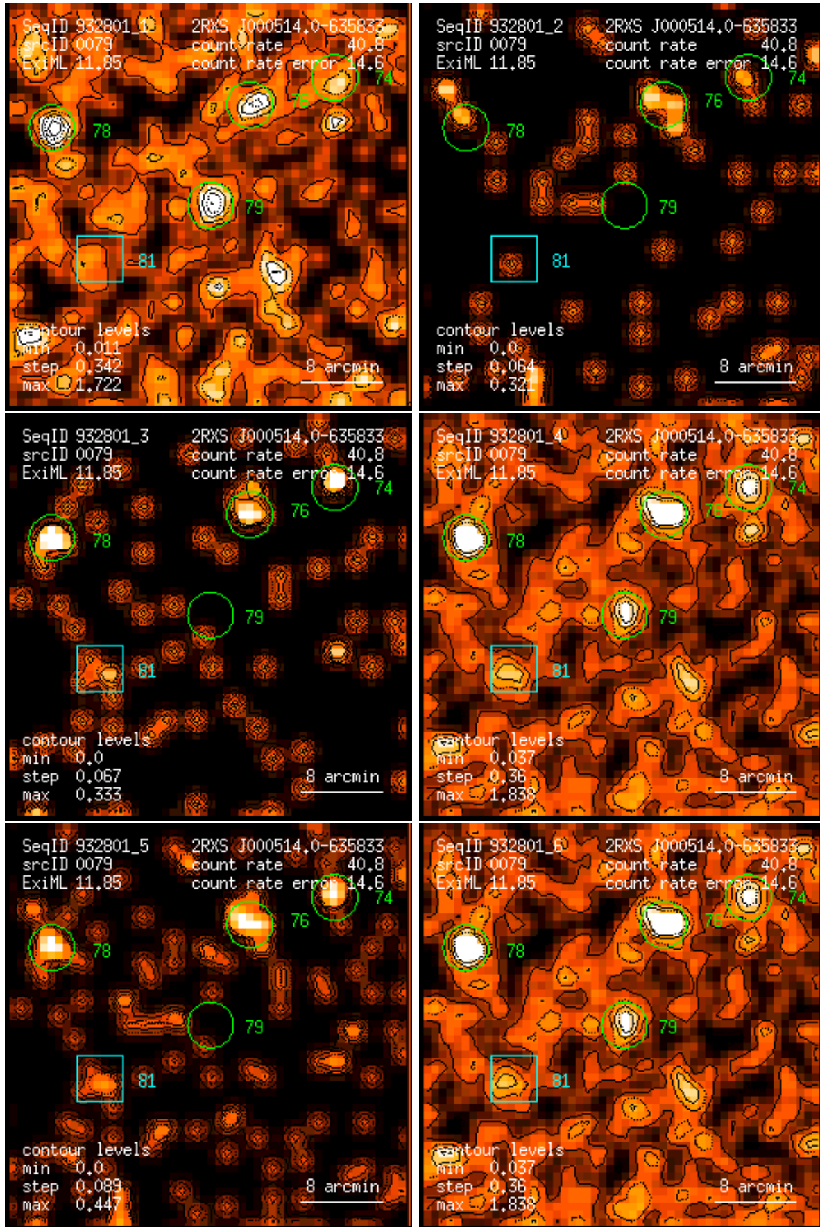
Figure 79: RASS 932801: detection 0079: band rate images, Gaussian filter: (1) PSPC channels 11 – 41, (2) 52 – 90, (3) 91 – 201, (4) 11 – 235, (5) 52 – 201, (6) 11 – 201. Broad band rates in counts/ks. Band rate contour levels in counts/ks/arcmin 2 .
