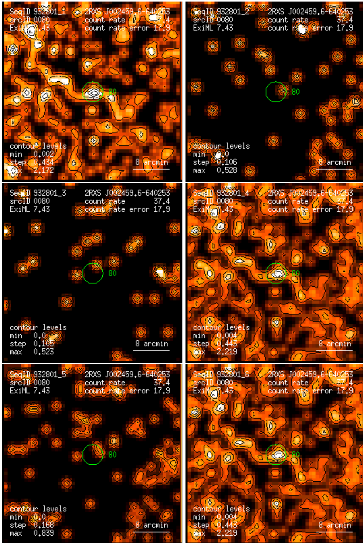
Figure 80: RASS 932801: detection 0080: band rate images, Gaussian filter: (1) PSPC channels 11 – 41, (2) 52 – 90, (3) 91 – 201, (4) 11 – 235, (5) 52 – 201, (6) 11 – 201. Broad band rates in counts/ks. Band rate contour levels in counts/ks/arcmin 2 .
