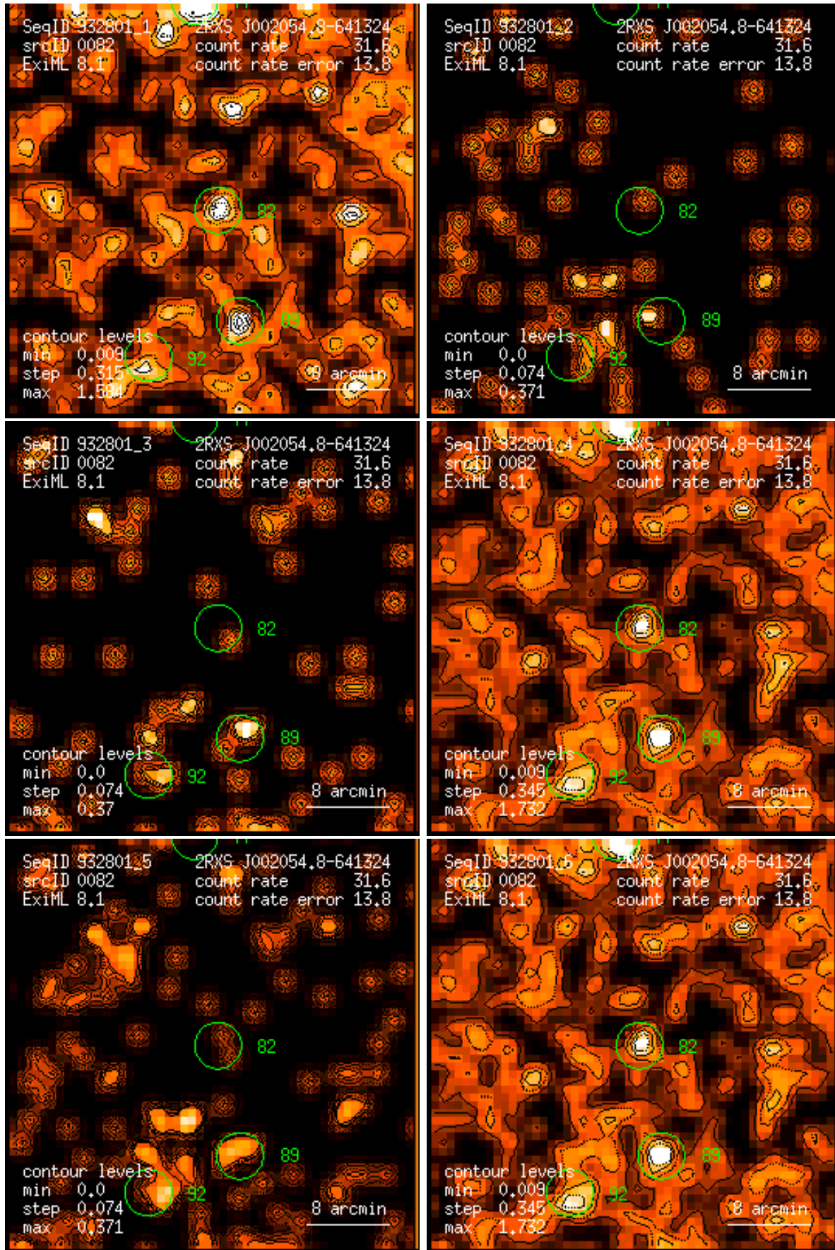
Figure 82: RASS 932801: detection 0082: band rate images, Gaussian filter: (1) PSPC channels 11 – 41, (2) 52 – 90, (3) 91 – 201, (4) 11 – 235, (5) 52 – 201, (6) 11 – 201. Broad band rates in counts/ks. Band rate contour levels in counts/ks/arcmin 2 .
