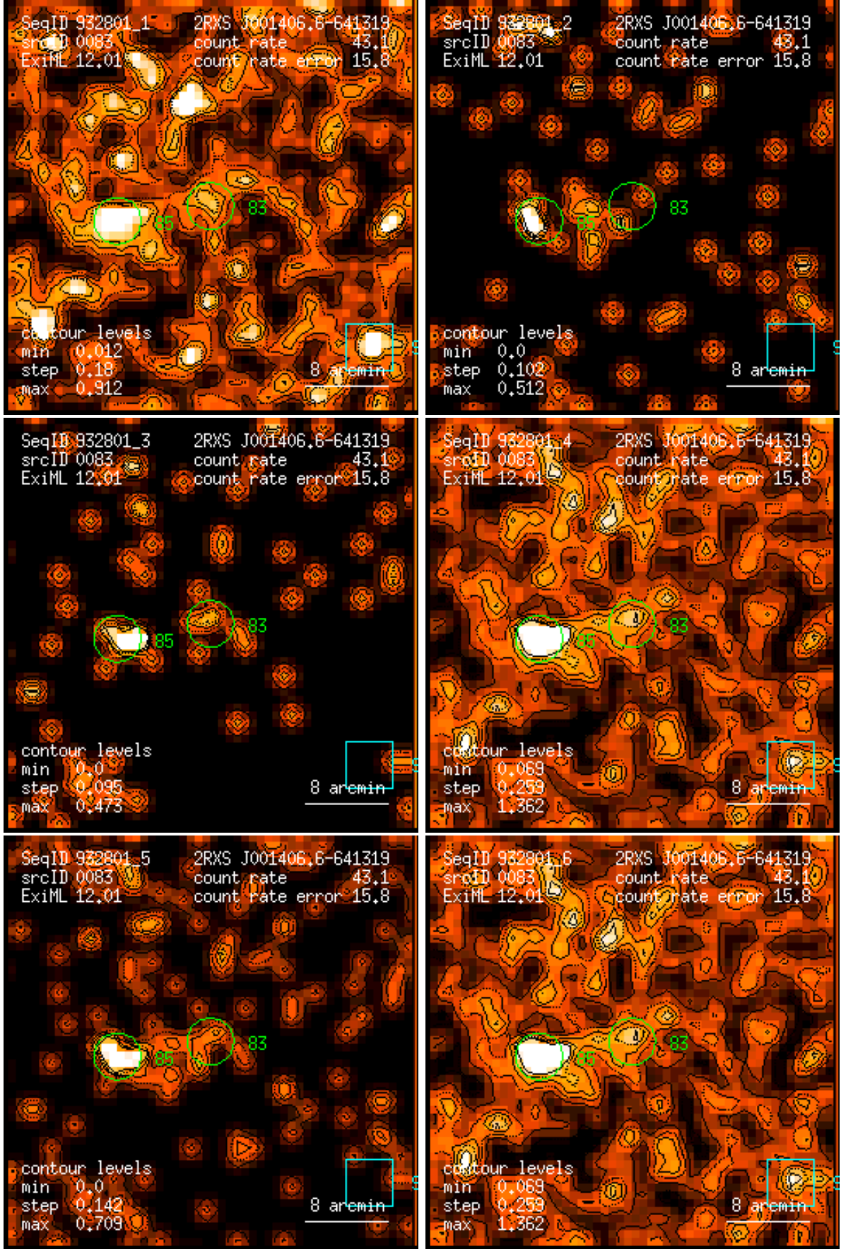
Figure 83: RASS 932801: detection 0083: band rate images, Gaussian filter: (1) PSPC channels 11 – 41, (2) 52 – 90, (3) 91 – 201, (4) 11 – 235, (5) 52 – 201, (6) 11 – 201. Broad band rates in counts/ks. Band rate contour levels in counts/ks/arcmin 2 .
