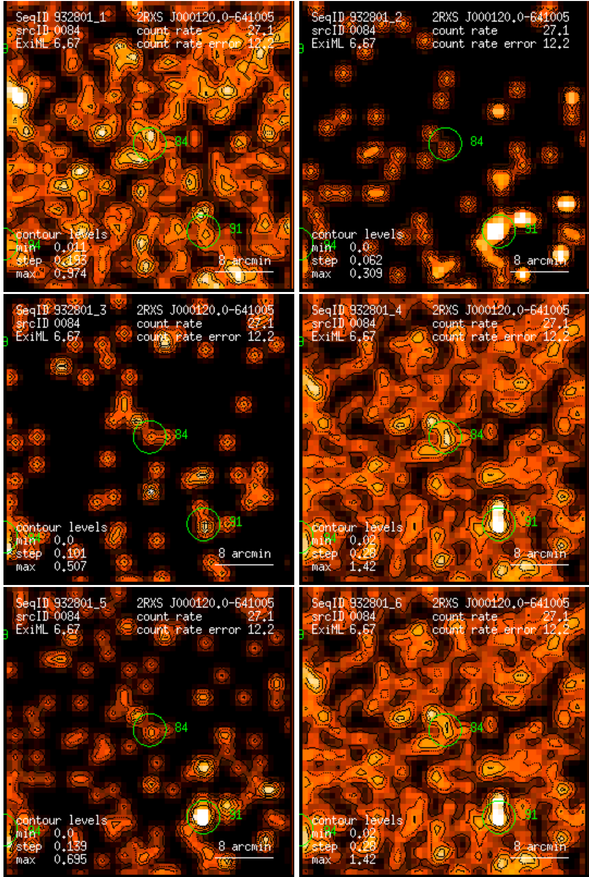
Figure 84: RASS 932801: detection 0084: band rate images, Gaussian filter: (1) PSPC channels 11 – 41, (2) 52 – 90, (3) 91 – 201, (4) 11 – 235, (5) 52 – 201, (6) 11 – 201. Broad band rates in counts/ks. Band rate contour levels in counts/ks/arcmin 2 .
