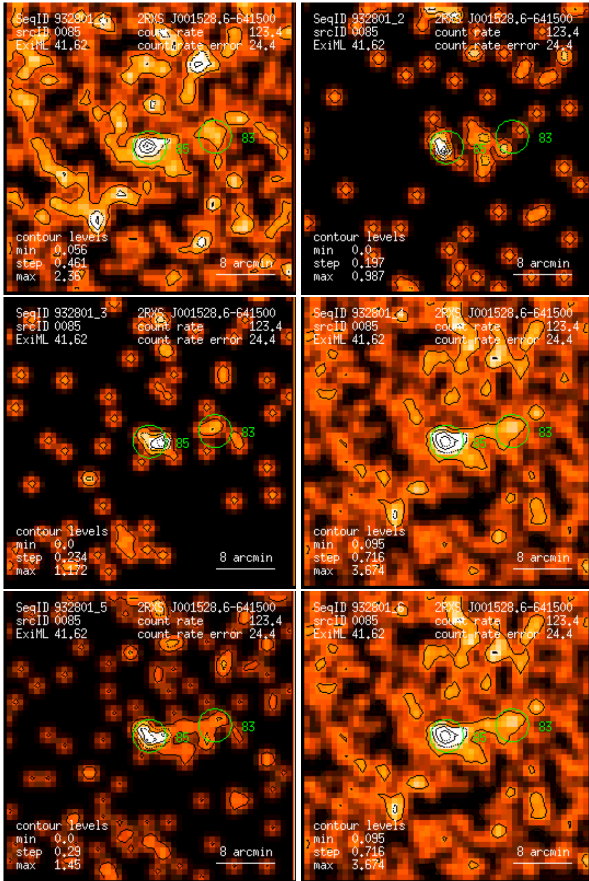
Figure 85: RASS 932801: detection 0085: band rate images, Gaussian filter: (1) PSPC channels 11 – 41, (2) 52 – 90, (3) 91 – 201, (4) 11 – 235, (5) 52 – 201, (6) 11 – 201. Broad band rates in counts/ks. Band rate contour levels in counts/ks/arcmin 2 .
