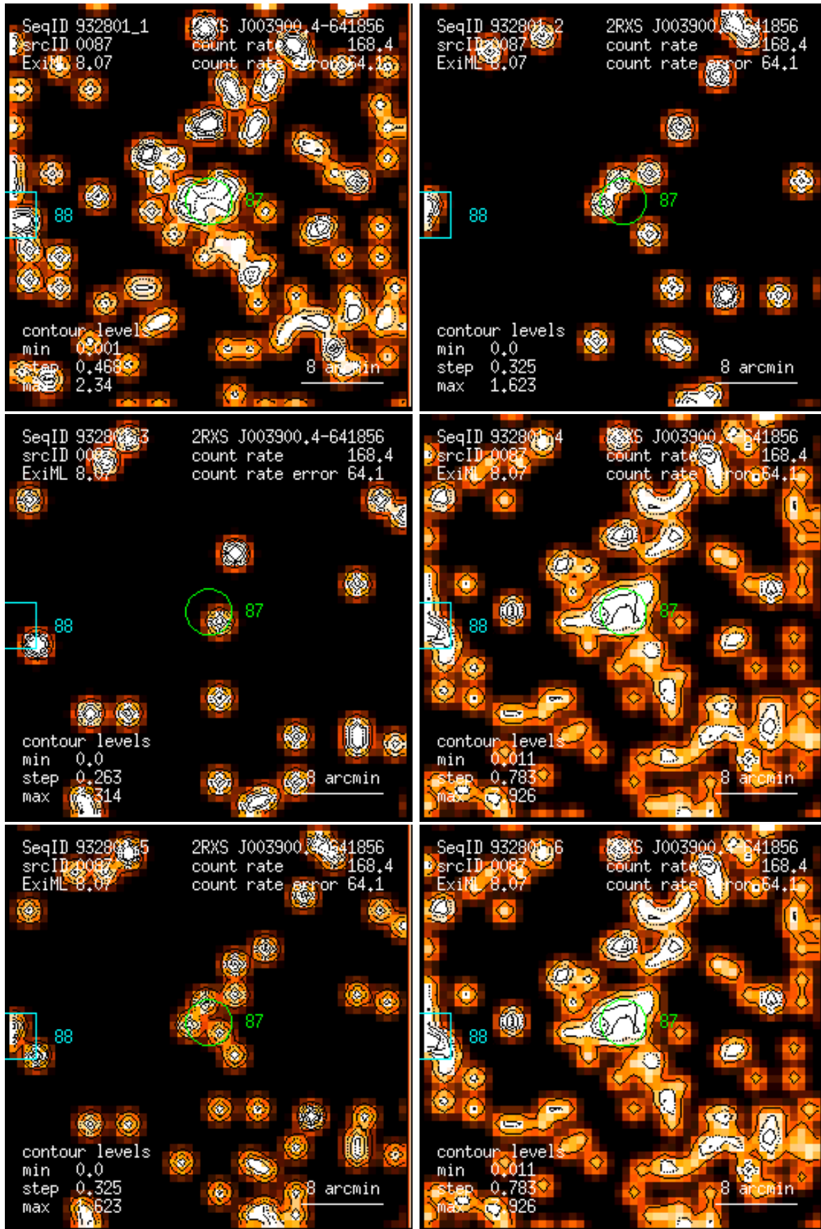
Figure 87: RASS 932801: detection 0087: band rate images, Gaussian filter: (1) PSPC channels 11 – 41, (2) 52 – 90, (3) 91 – 201, (4) 11 – 235, (5) 52 – 201, (6) 11 – 201. Broad band rates in counts/ks. Band rate contour levels in counts/ks/arcmin 2 .
