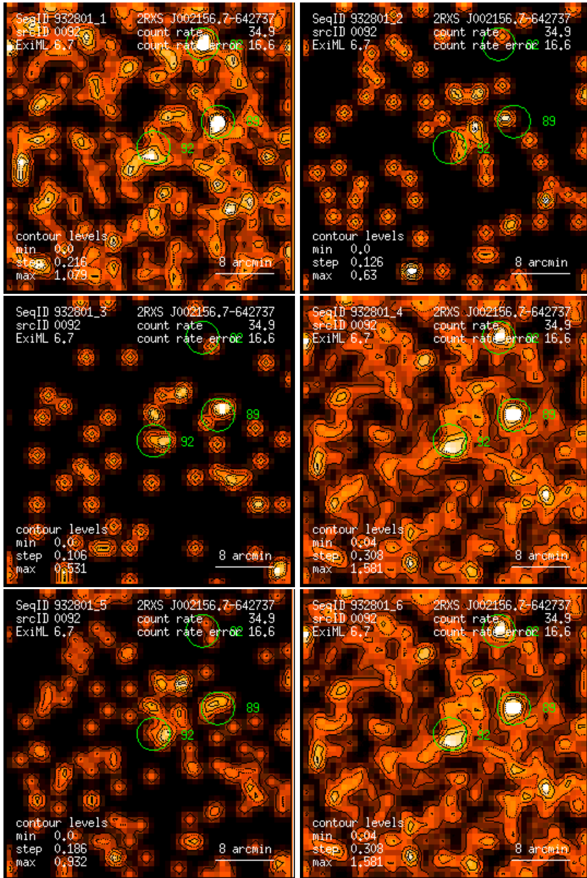
Figure 92: RASS 932801: detection 0092: band rate images, Gaussian filter: (1) PSPC channels 11 – 41, (2) 52 – 90, (3) 91 – 201, (4) 11 – 235, (5) 52 – 201, (6) 11 – 201. Broad band rates in counts/ks. Band rate contour levels in counts/ks/arcmin 2 .
