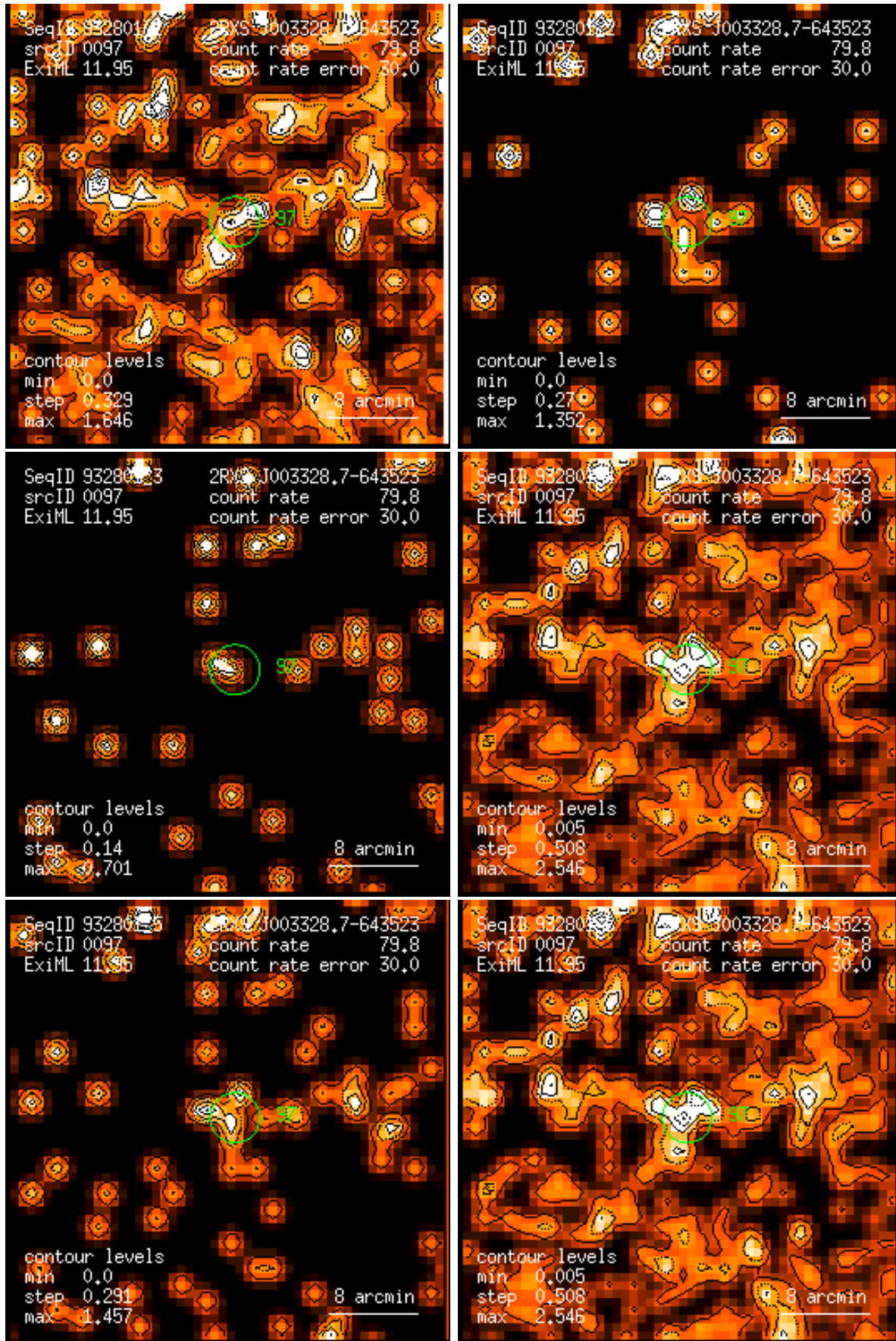
Figure 97: RASS 932801: detection 0097: band rate images, Gaussian filter: (1) PSPC channels 11 – 41, (2) 52 – 90, (3) 91 – 201, (4) 11 – 235, (5) 52 – 201, (6) 11 – 201. Broad band rates in counts/ks. Band rate contour levels in counts/ks/arcmin 2 .
