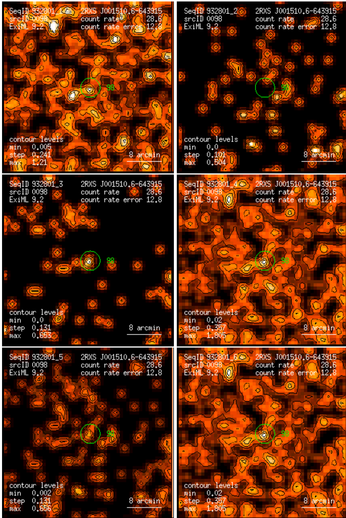
Figure 98: RASS 932801: detection 0098: band rate images, Gaussian filter: (1) PSPC channels 11 – 41, (2) 52 – 90, (3) 91 – 201, (4) 11 – 235, (5) 52 – 201, (6) 11 – 201. Broad band rates in counts/ks. Band rate contour levels in counts/ks/arcmin 2 .
