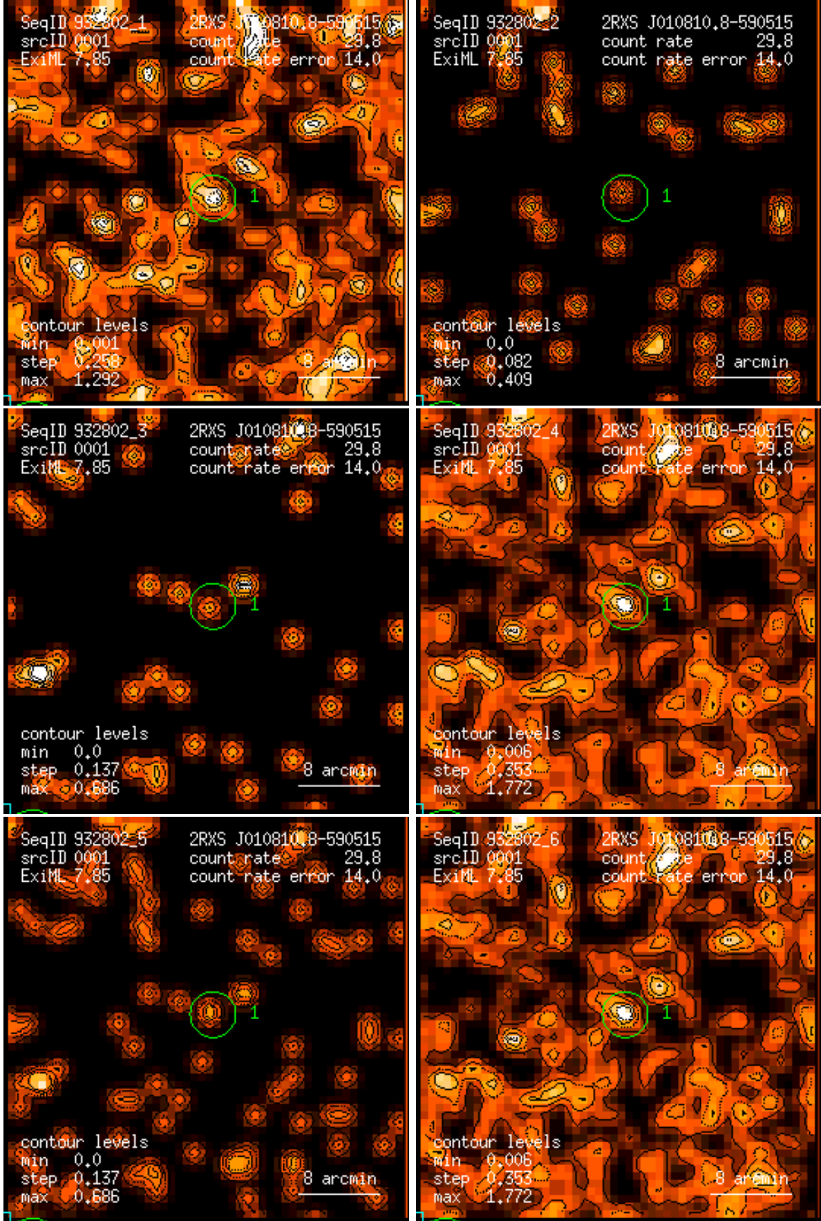
Figure 1: RASS 932802: detection 0001: band rate images, Gaussian filter: (1) PSPC channels 11 – 41, (2) 52 – 90, (3) 91 – 201, (4) 11 – 235, (5) 52 – 201, (6) 11 – 201. Broad band rates in counts/ks. Band rate contour levels in counts/ks/arcmin 2 .
