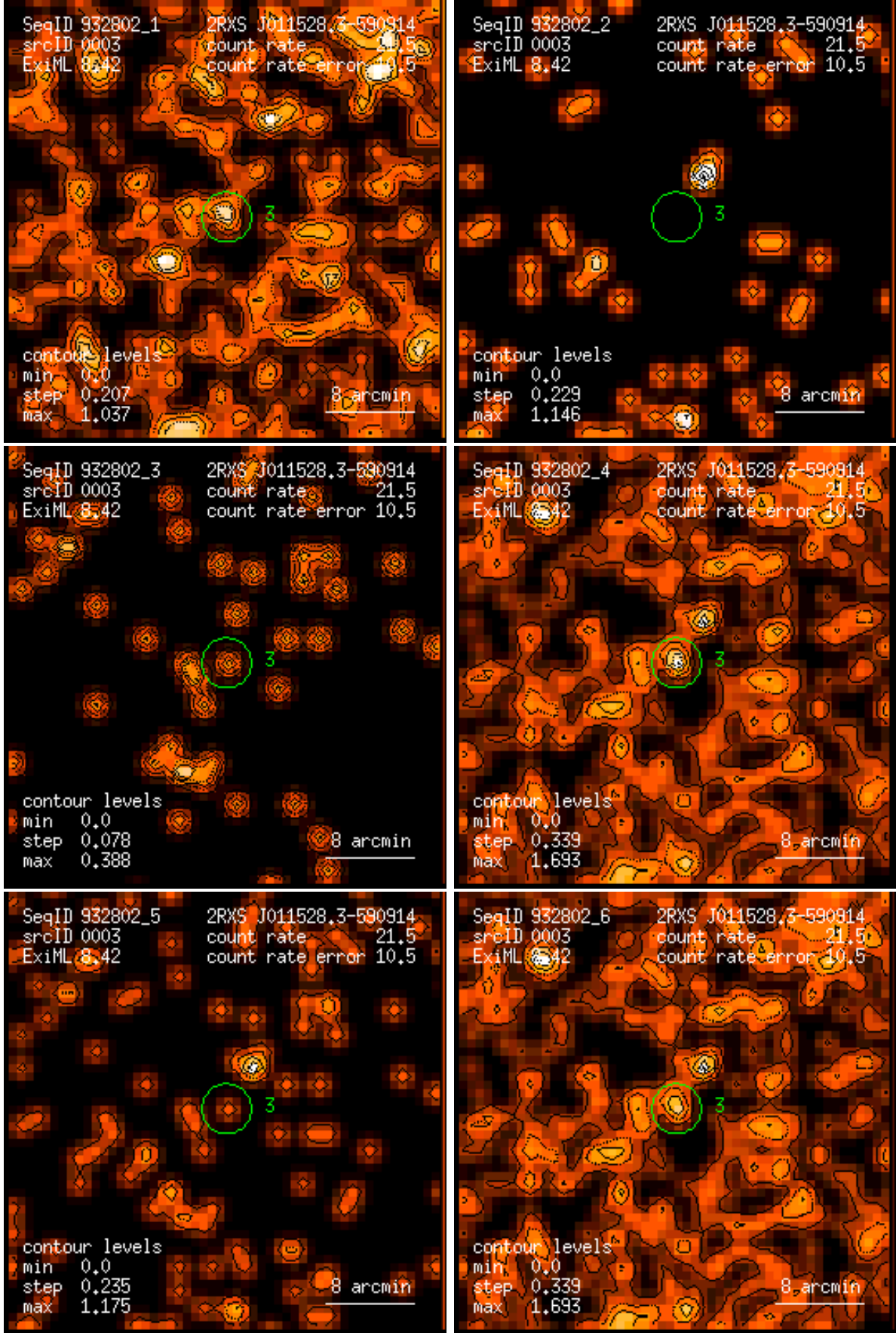
Figure 3: RASS 932802: detection 0003: band rate images, Gaussian filter: (1) PSPC channels 11 – 41, (2) 52 – 90, (3) 91 – 201, (4) 11 – 235, (5) 52 – 201, (6) 11 – 201. Broad band rates in counts/ks. Band rate contour levels in counts/ks/arcmin 2 .
