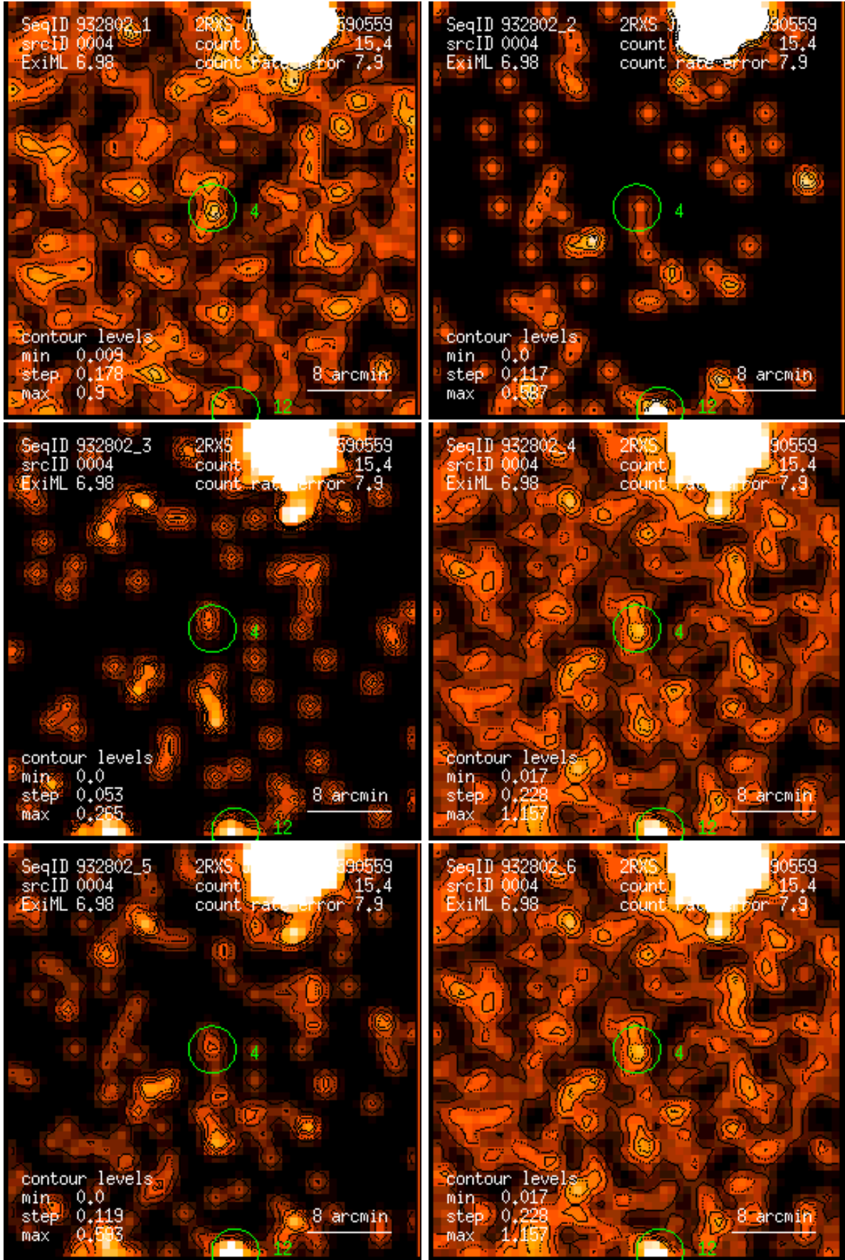
Figure 4: RASS 932802: detection 0004: band rate images, Gaussian filter: (1) PSPC channels 11 – 41, (2) 52 – 90, (3) 91 – 201, (4) 11 – 235, (5) 52 – 201, (6) 11 – 201. Broad band rates in counts/ks. Band rate contour levels in counts/ks/arcmin 2 .
