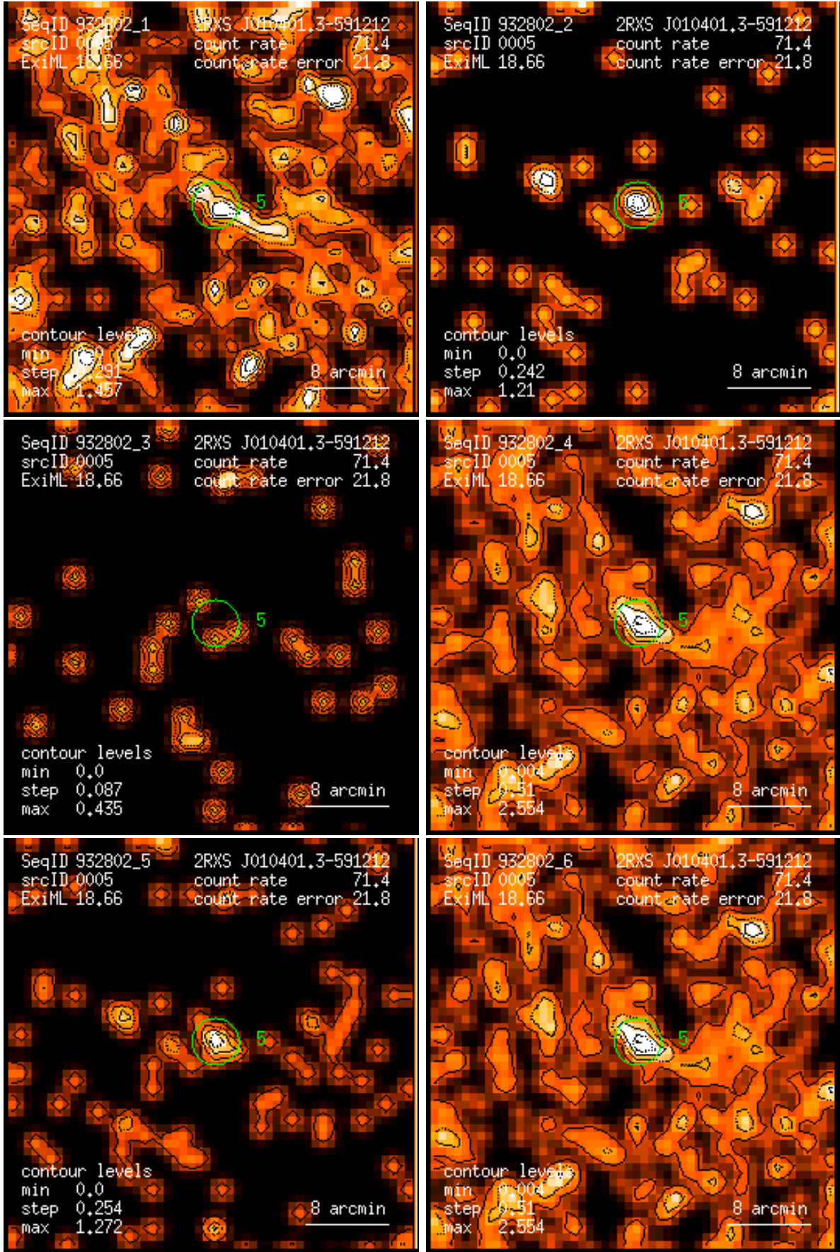
Figure 5: RASS 932802: detection 0005: band rate images, Gaussian filter: (1) PSPC channels 11 – 41, (2) 52 – 90, (3) 91 – 201, (4) 11 – 235, (5) 52 – 201, (6) 11 – 201. Broad band rates in counts/ks. Band rate contour levels in counts/ks/arcmin 2 .
