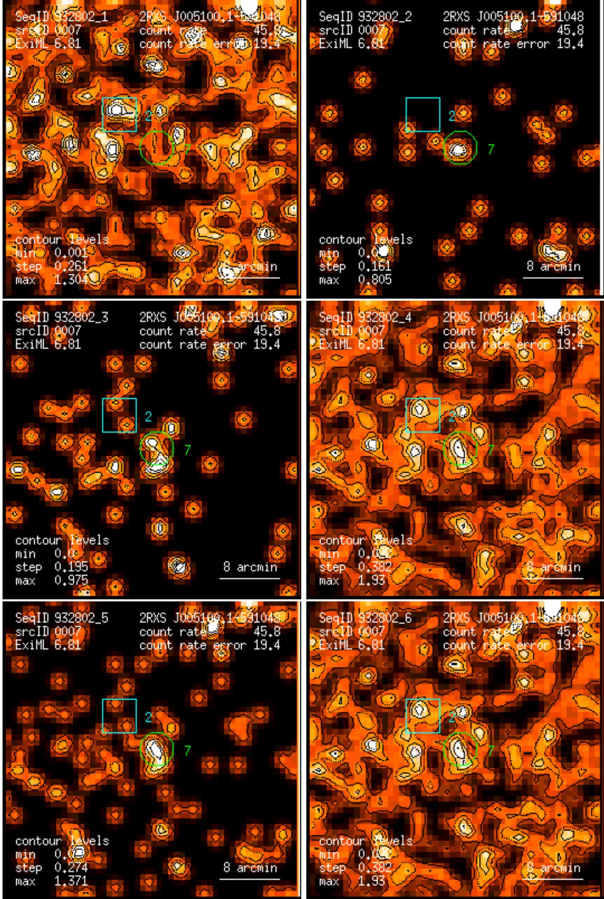
Figure 7: RASS 932802: detection 0007: band rate images, Gaussian filter: (1) PSPC channels 11 – 41, (2) 52 – 90, (3) 91 – 201, (4) 11 – 235, (5) 52 – 201, (6) 11 – 201. Broad band rates in counts/ks. Band rate contour levels in counts/ks/arcmin 2 .
