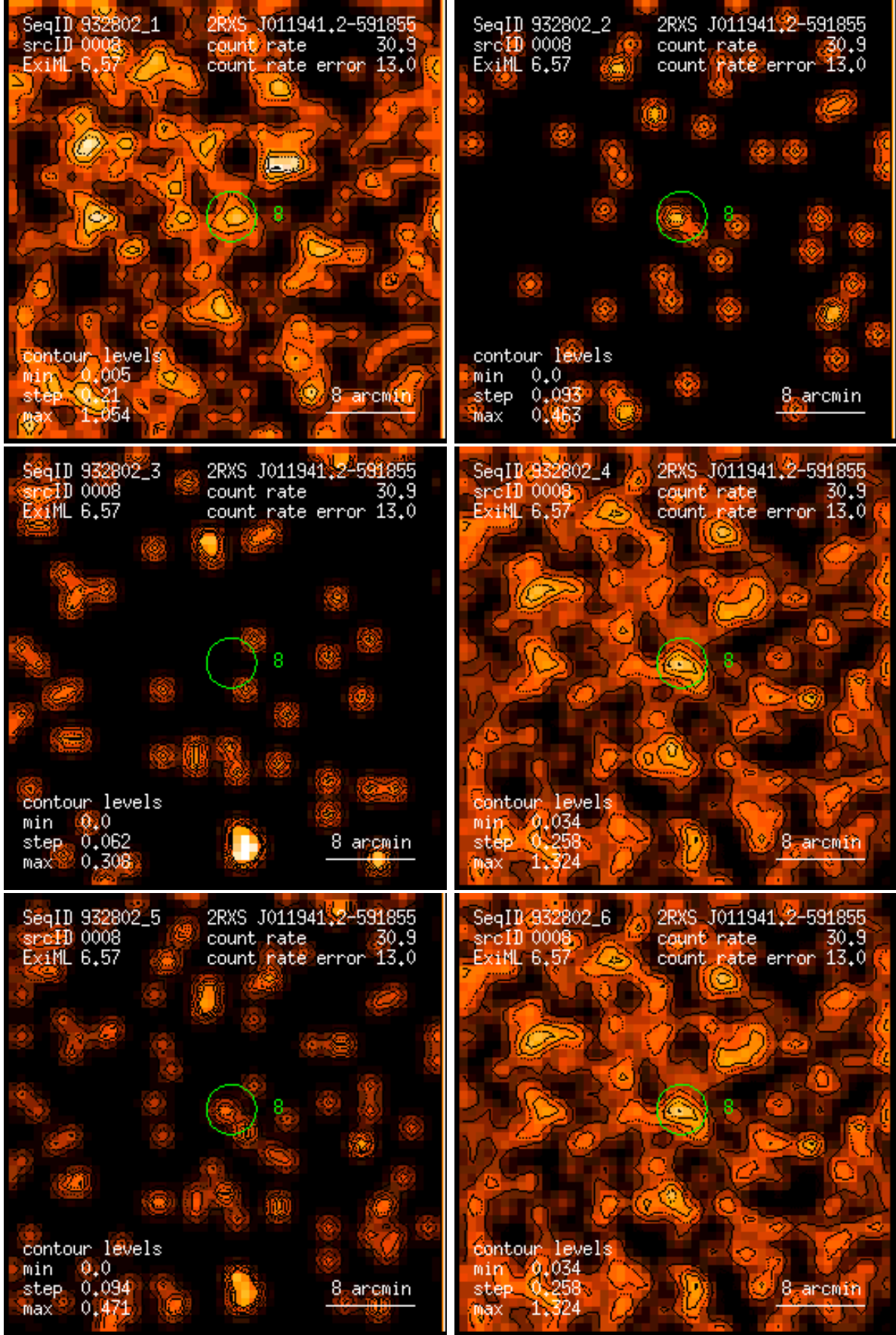
Figure 8: RASS 932802: detection 0008: band rate images, Gaussian filter: (1) PSPC channels 11 – 41, (2) 52 – 90, (3) 91 – 201, (4) 11 – 235, (5) 52 – 201, (6) 11 – 201. Broad band rates in counts/ks. Band rate contour levels in counts/ks/arcmin 2 .
