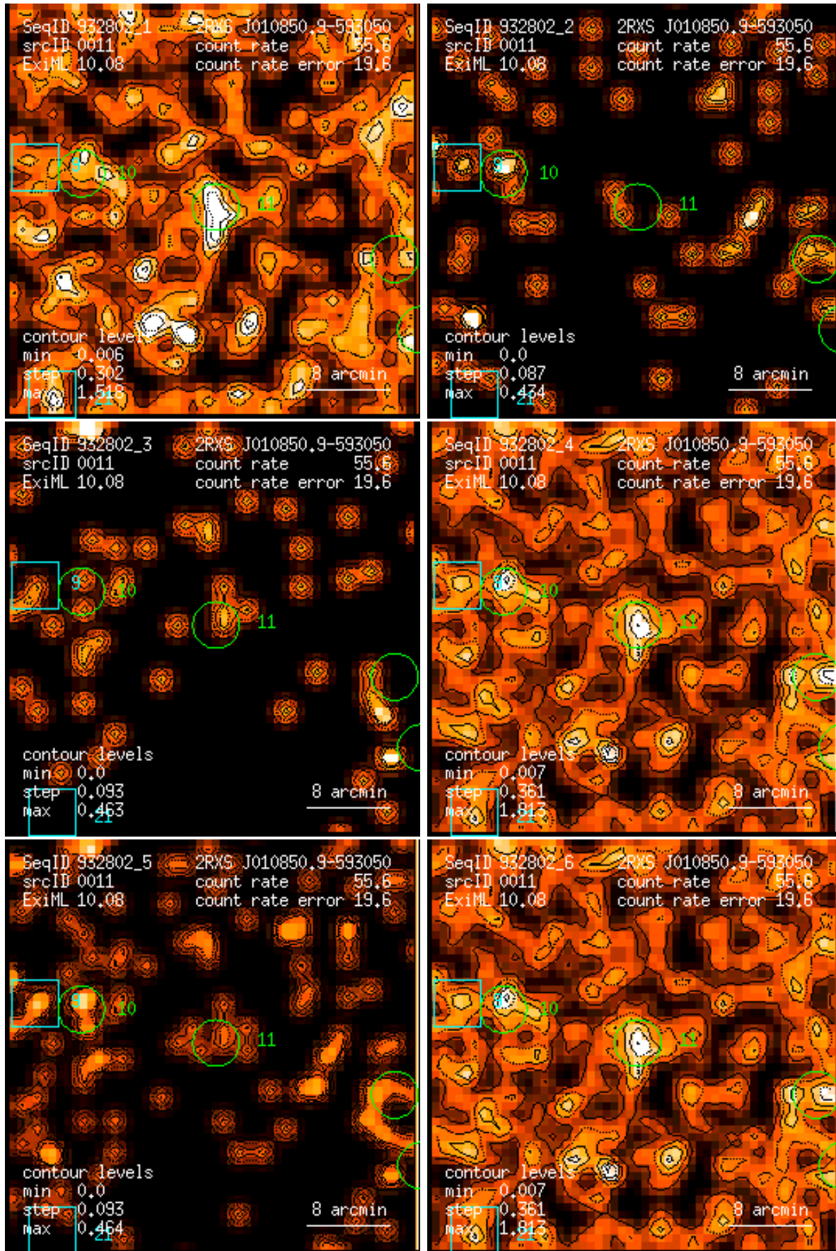
Figure 11: RASS 932802: detection 0011: band rate images, Gaussian filter: (1) PSPC channels 11 – 41, (2) 52 – 90, (3) 91 – 201, (4) 11 – 235, (5) 52 – 201, (6) 11 – 201. Broad band rates in counts/ks. Band rate contour levels in counts/ks/arcmin 2 .
