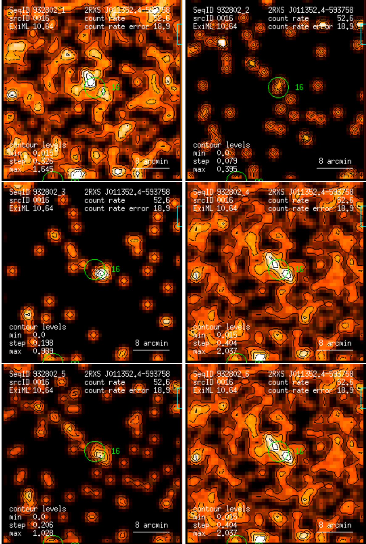
Figure 16: RASS 932802: detection 0016: band rate images, Gaussian filter: (1) PSPC channels 11 – 41, (2) 52 – 90, (3) 91 – 201, (4) 11 – 235, (5) 52 – 201, (6) 11 – 201. Broad band rates in counts/ks. Band rate contour levels in counts/ks/arcmin 2 .
