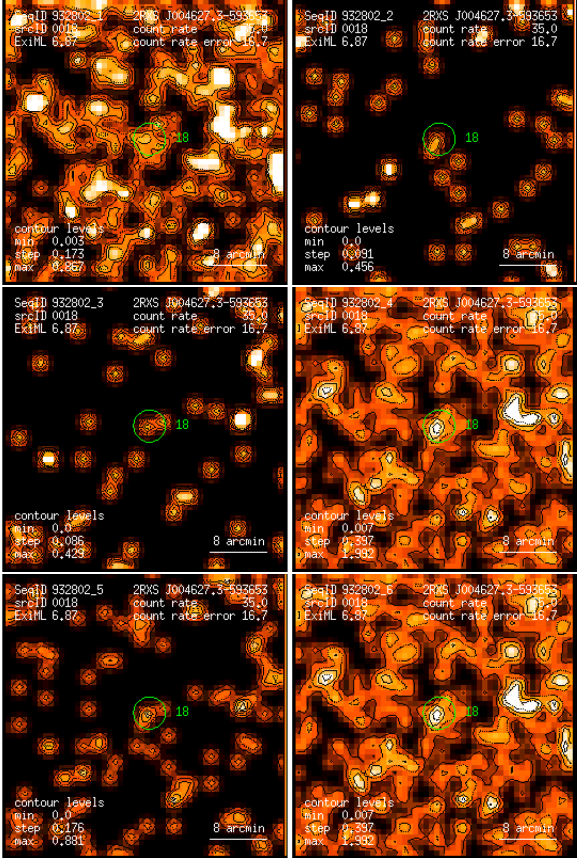
Figure 18: RASS 932802: detection 0018: band rate images, Gaussian filter: (1) PSPC channels 11 – 41, (2) 52 – 90, (3) 91 – 201, (4) 11 – 235, (5) 52 – 201, (6) 11 – 201. Broad band rates in counts/ks. Band rate contour levels in counts/ks/arcmin 2 .
