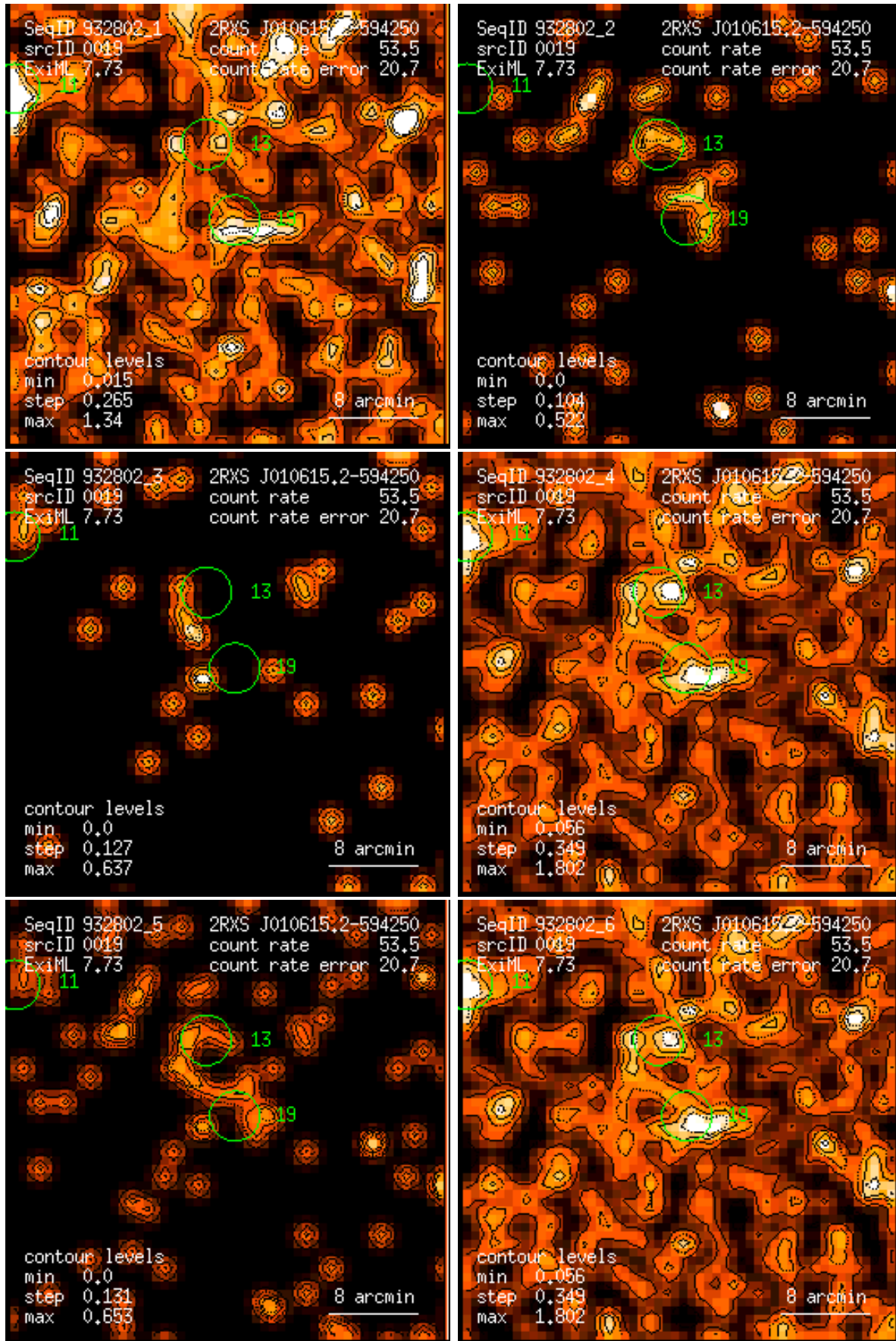
Figure 19: RASS 932802: detection 0019: band rate images, Gaussian filter: (1) PSPC channels 11 – 41, (2) 52 – 90, (3) 91 – 201, (4) 11 – 235, (5) 52 – 201, (6) 11 – 201. Broad band rates in counts/ks. Band rate contour levels in counts/ks/arcmin 2 .
