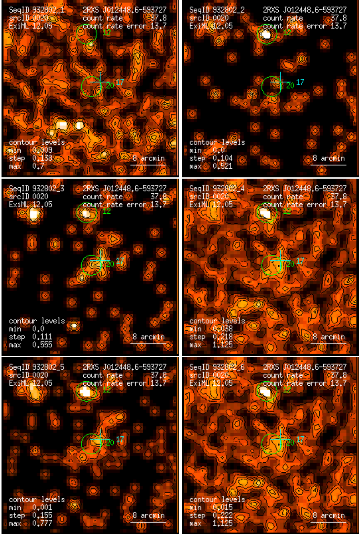
Figure 20: RASS 932802: detection 0020: band rate images, Gaussian filter: (1) PSPC channels 11 – 41, (2) 52 – 90, (3) 91 – 201, (4) 11 – 235, (5) 52 – 201, (6) 11 – 201. Broad band rates in counts/ks. Band rate contour levels in counts/ks/arcmin 2 .
