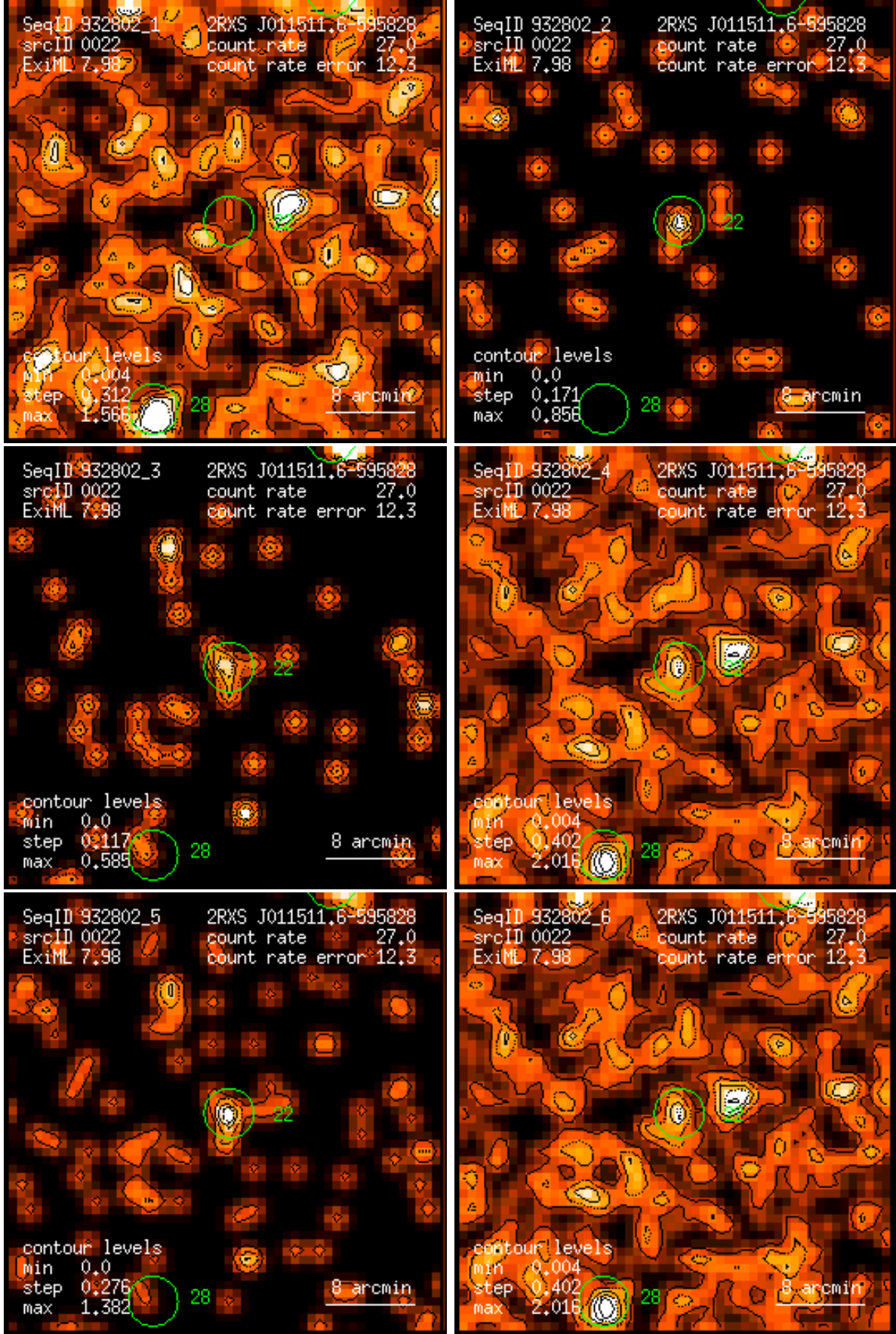
Figure 22: RASS 932802: detection 0022: band rate images, Gaussian filter: (1) PSPC channels 11 – 41, (2) 52 – 90, (3) 91 – 201, (4) 11 – 235, (5) 52 – 201, (6) 11 – 201. Broad band rates in counts/ks. Band rate contour levels in counts/ks/arcmin 2 .
