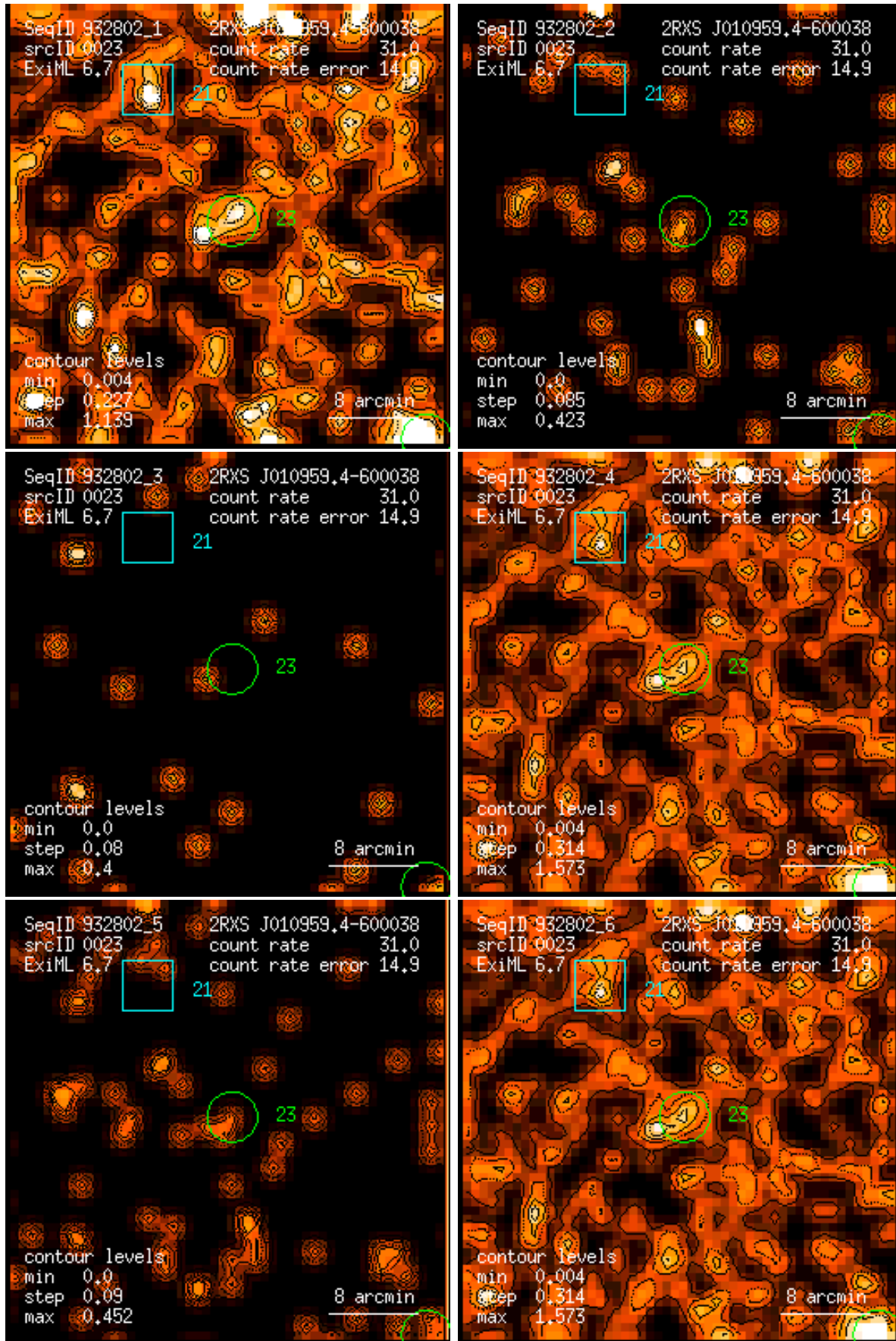
Figure 23: RASS 932802: detection 0023: band rate images, Gaussian filter: (1) PSPC channels 11 – 41, (2) 52 – 90, (3) 91 – 201, (4) 11 – 235, (5) 52 – 201, (6) 11 – 201. Broad band rates in counts/ks. Band rate contour levels in counts/ks/arcmin 2 .
