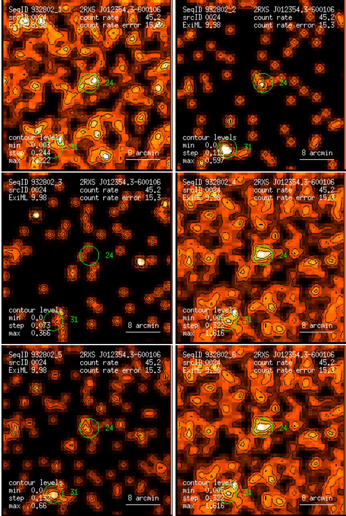
Figure 24: RASS 932802: detection 0024: band rate images, Gaussian filter: (1) PSPC channels 11 – 41, (2) 52 – 90, (3) 91 – 201, (4) 11 – 235, (5) 52 – 201, (6) 11 – 201. Broad band rates in counts/ks. Band rate contour levels in counts/ks/arcmin 2 .
