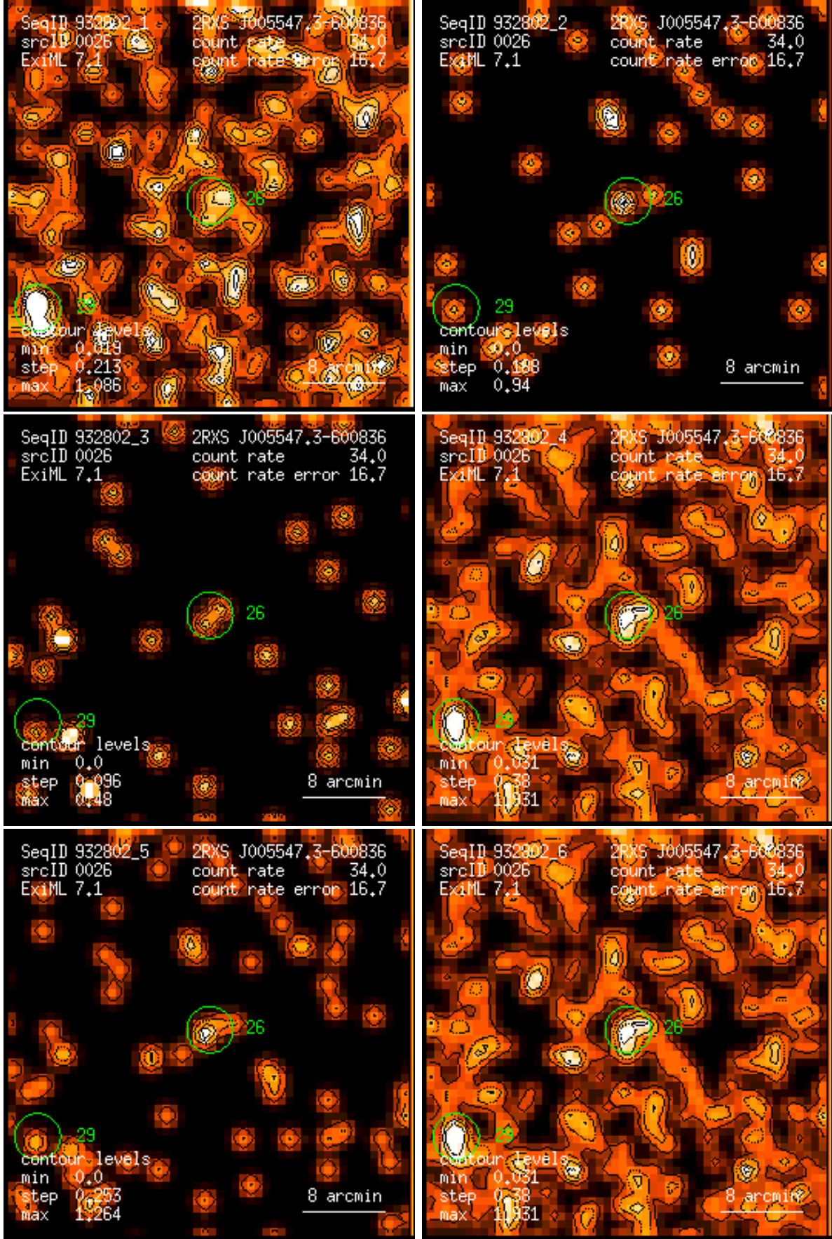
Figure 26: RASS 932802: detection 0026: band rate images, Gaussian filter: (1) PSPC channels 11 – 41, (2) 52 – 90, (3) 91 – 201, (4) 11 – 235, (5) 52 – 201, (6) 11 – 201. Broad band rates in counts/ks. Band rate contour levels in counts/ks/arcmin 2 .
