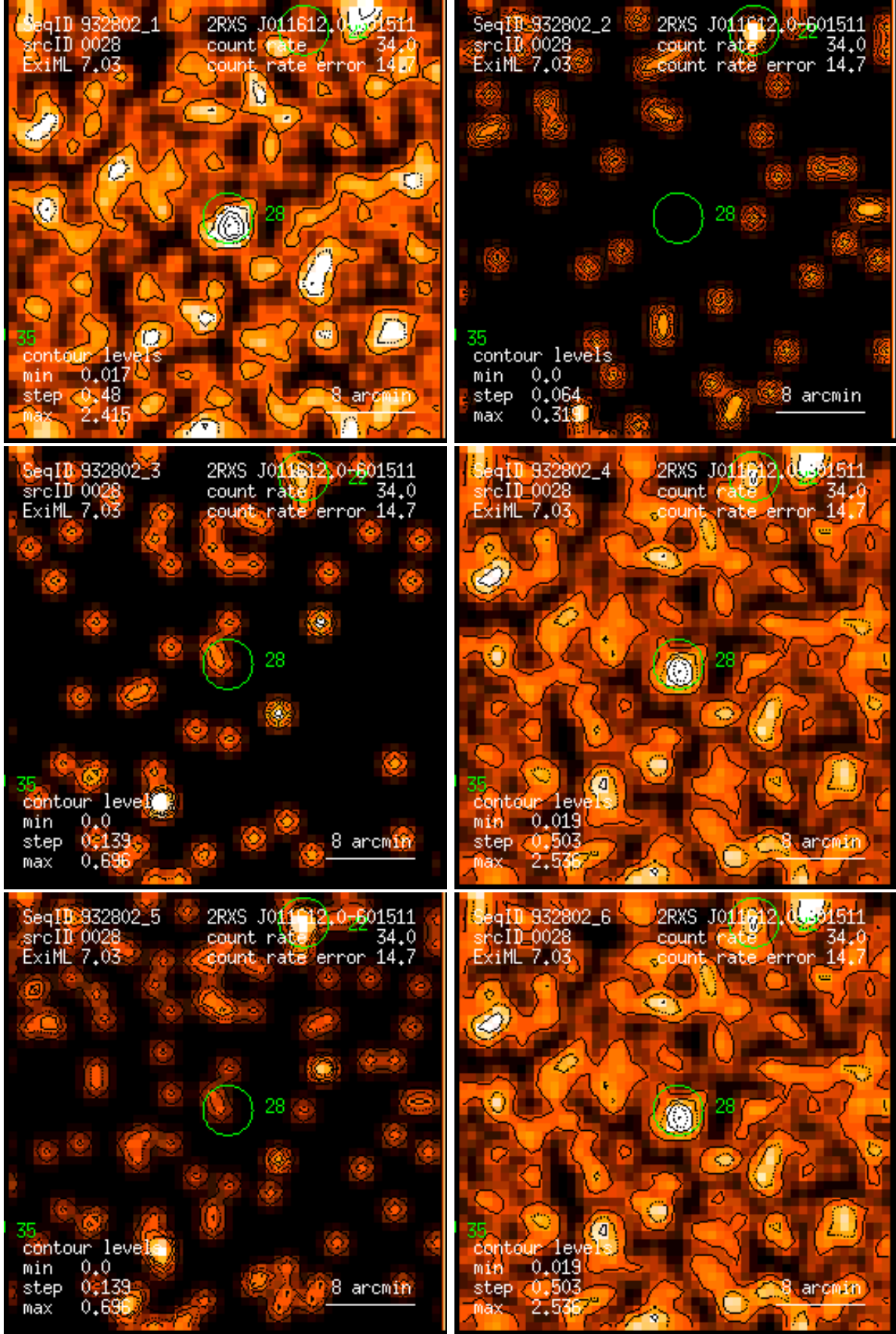
Figure 28: RASS 932802: detection 0028: band rate images, Gaussian filter: (1) PSPC channels 11 – 41, (2) 52 – 90, (3) 91 – 201, (4) 11 – 235, (5) 52 – 201, (6) 11 – 201. Broad band rates in counts/ks. Band rate contour levels in counts/ks/arcmin 2 .
