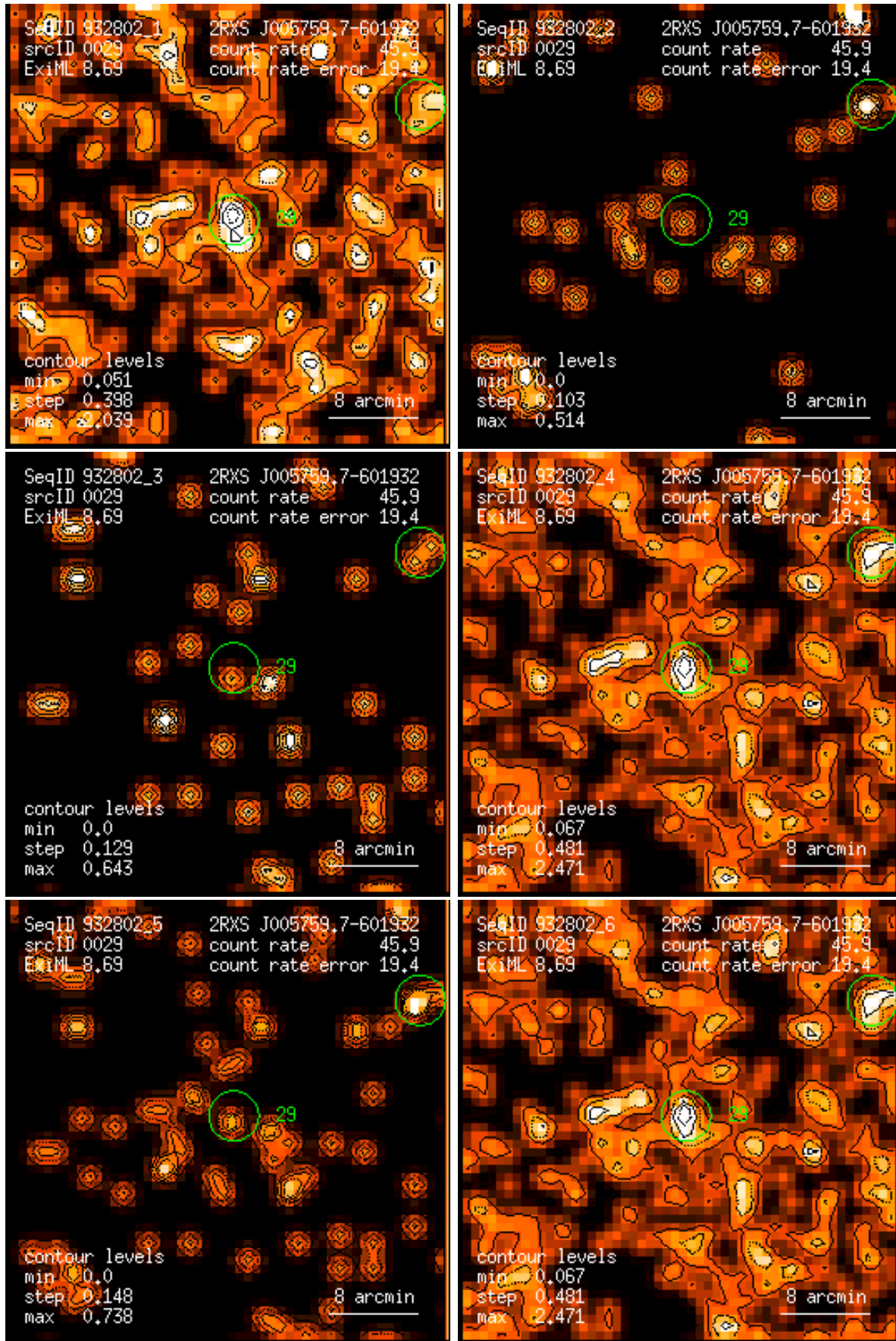
Figure 29: RASS 932802: detection 0029: band rate images, Gaussian filter: (1) PSPC channels 11 – 41, (2) 52 – 90, (3) 91 – 201, (4) 11 – 235, (5) 52 – 201, (6) 11 – 201. Broad band rates in counts/ks. Band rate contour levels in counts/ks/arcmin 2 .
