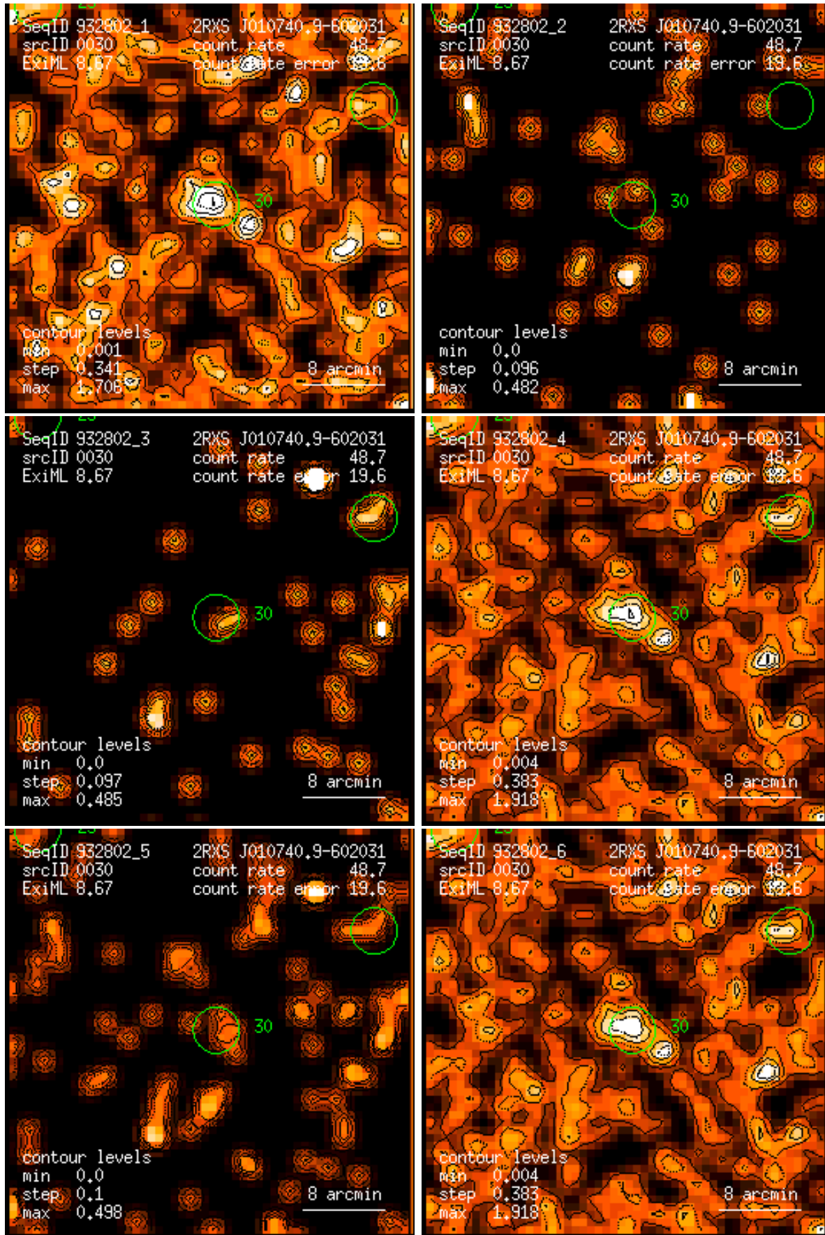
Figure 30: RASS 932802: detection 0030: band rate images, Gaussian filter: (1) PSPC channels 11 – 41, (2) 52 – 90, (3) 91 – 201, (4) 11 – 235, (5) 52 – 201, (6) 11 – 201. Broad band rates in counts/ks. Band rate contour levels in counts/ks/arcmin 2 .
