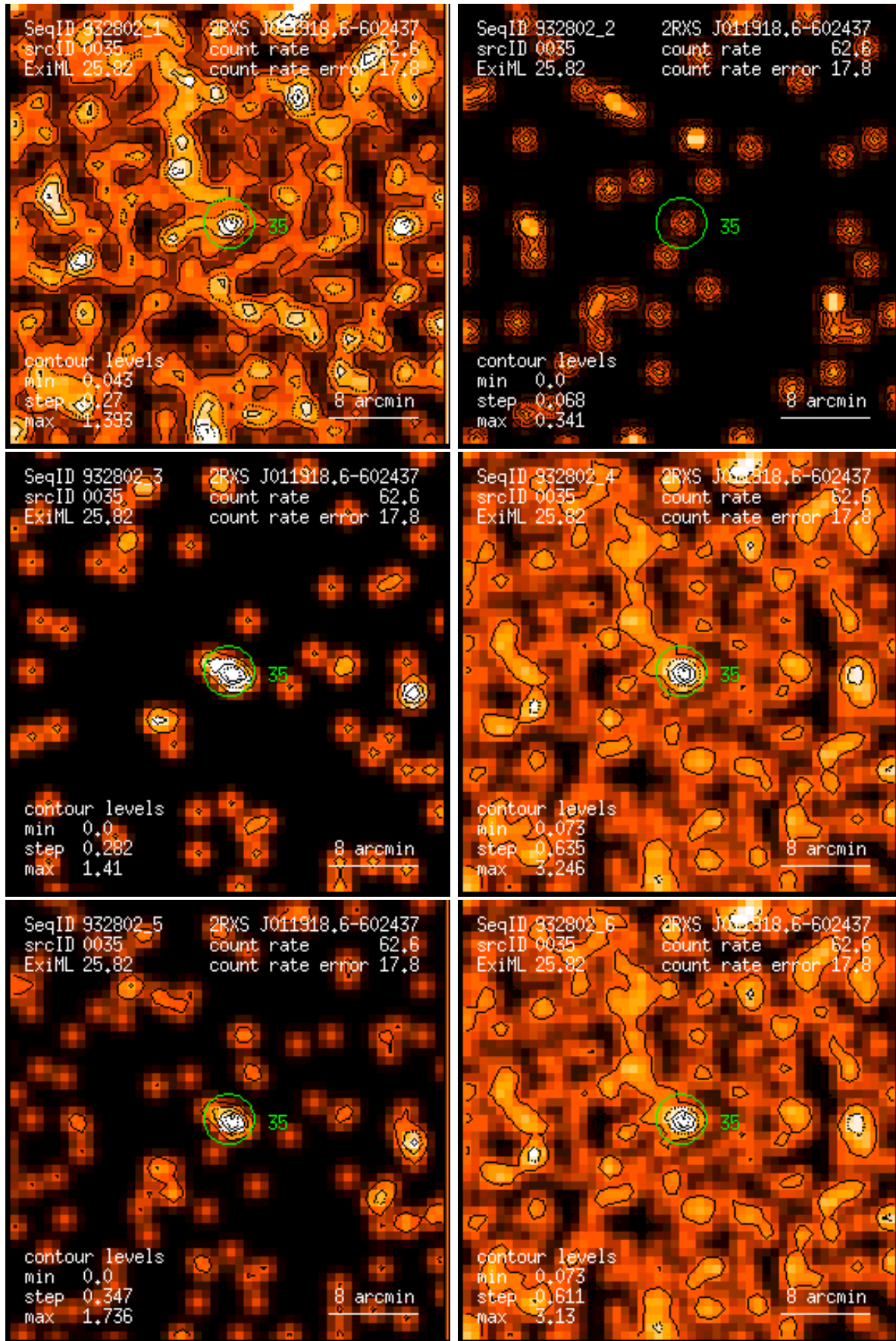
Figure 35: RASS 932802: detection 0035: band rate images, Gaussian filter: (1) PSPC channels 11 – 41, (2) 52 – 90, (3) 91 – 201, (4) 11 – 235, (5) 52 – 201, (6) 11 – 201. Broad band rates in counts/ks. Band rate contour levels in counts/ks/arcmin 2 .
