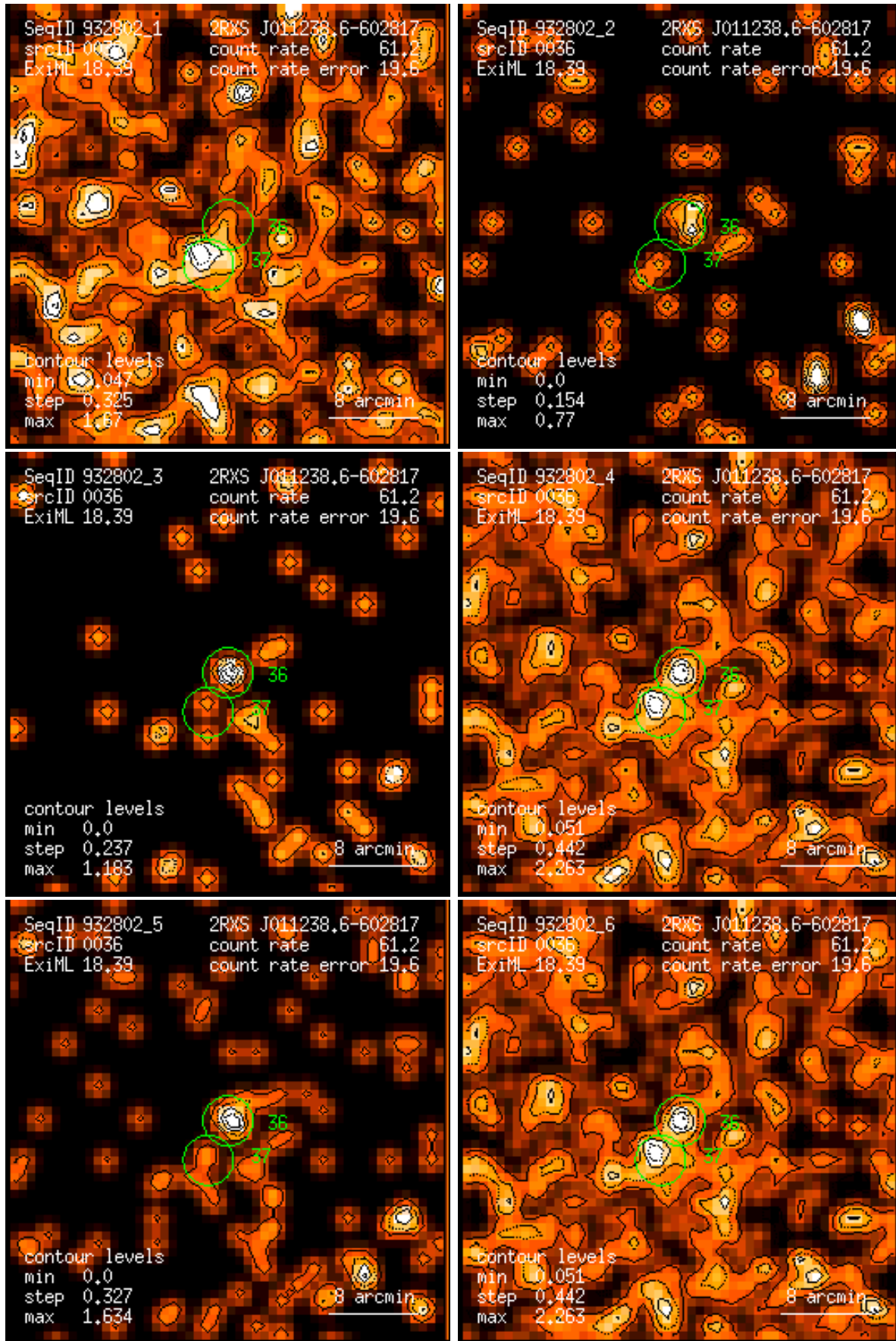
Figure 36: RASS 932802: detection 0036: band rate images, Gaussian filter: (1) PSPC channels 11 – 41, (2) 52 – 90, (3) 91 – 201, (4) 11 – 235, (5) 52 – 201, (6) 11 – 201. Broad band rates in counts/ks. Band rate contour levels in counts/ks/arcmin 2 .
