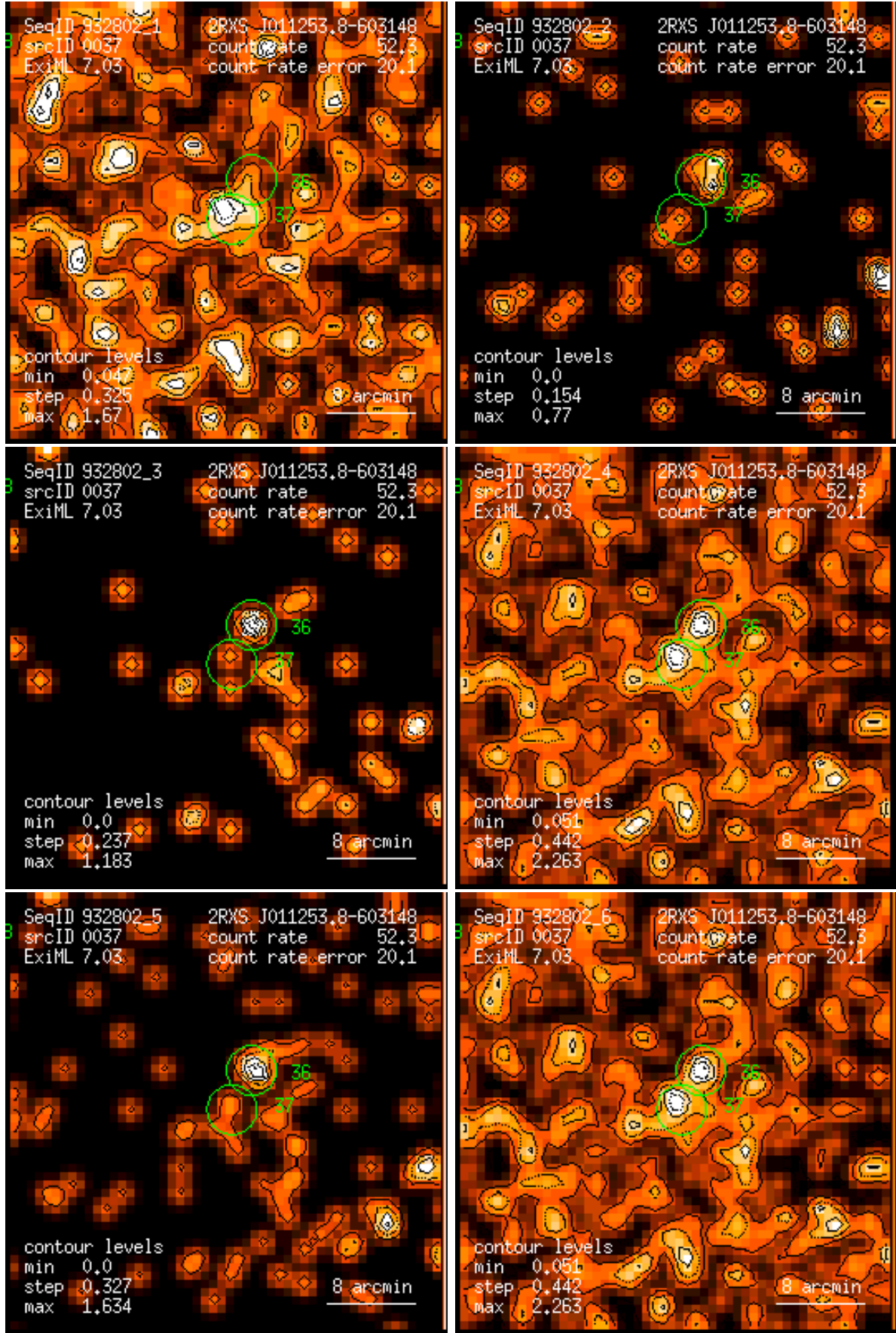
Figure 37: RASS 932802: detection 0037: band rate images, Gaussian filter: (1) PSPC channels 11 – 41, (2) 52 – 90, (3) 91 – 201, (4) 11 – 235, (5) 52 – 201, (6) 11 – 201. Broad band rates in counts/ks. Band rate contour levels in counts/ks/arcmin 2 .
