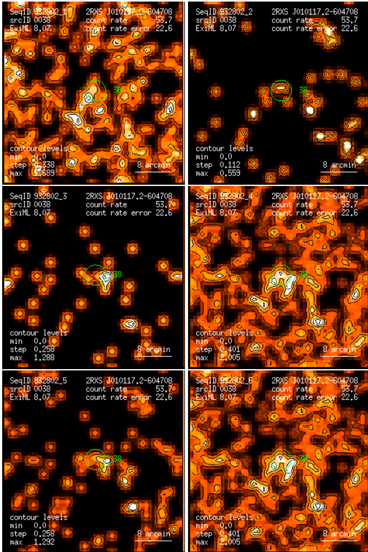
Figure 38: RASS 932802: detection 0038: band rate images, Gaussian filter: (1) PSPC channels 11 – 41, (2) 52 – 90, (3) 91 – 201, (4) 11 – 235, (5) 52 – 201, (6) 11 – 201. Broad band rates in counts/ks. Band rate contour levels in counts/ks/arcmin 2 .
