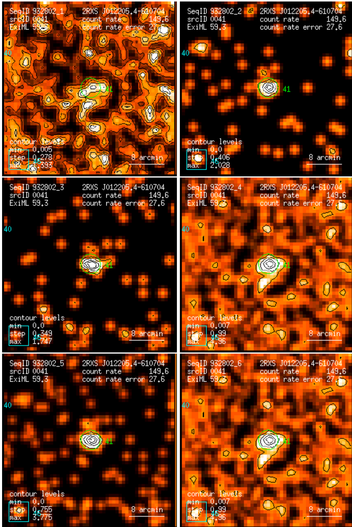
Figure 41: RASS 932802: detection 0041: band rate images, Gaussian filter: (1) PSPC channels 11 – 41, (2) 52 – 90, (3) 91 – 201, (4) 11 – 235, (5) 52 – 201, (6) 11 – 201. Broad band rates in counts/ks. Band rate contour levels in counts/ks/arcmin 2 .
