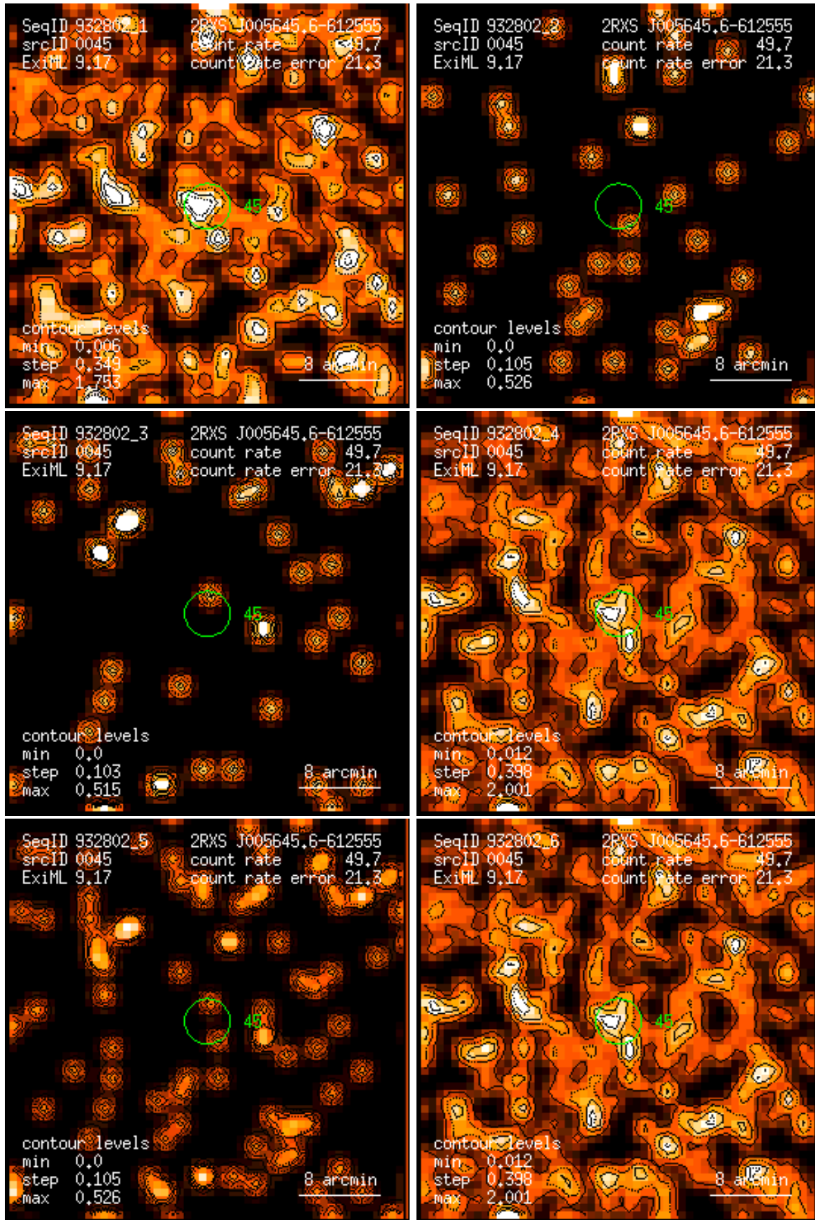
Figure 45: RASS 932802: detection 0045: band rate images, Gaussian filter: (1) PSPC channels 11 – 41, (2) 52 – 90, (3) 91 – 201, (4) 11 – 235, (5) 52 – 201, (6) 11 – 201. Broad band rates in counts/ks. Band rate contour levels in counts/ks/arcmin 2 .
