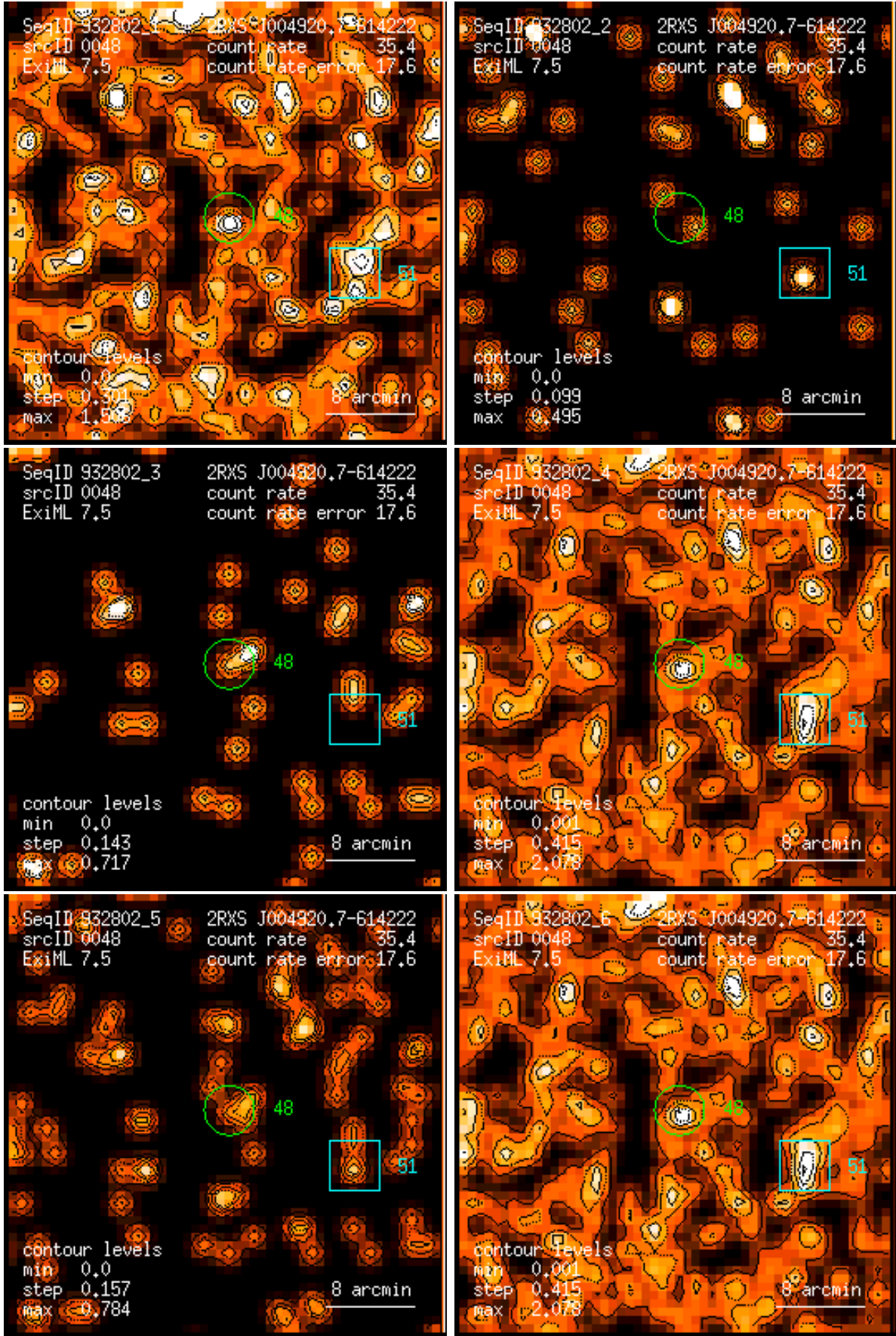
Figure 48: RASS 932802: detection 0048: band rate images, Gaussian filter: (1) PSPC channels 11 – 41, (2) 52 – 90, (3) 91 – 201, (4) 11 – 235, (5) 52 – 201, (6) 11 – 201. Broad band rates in counts/ks. Band rate contour levels in counts/ks/arcmin 2 .
