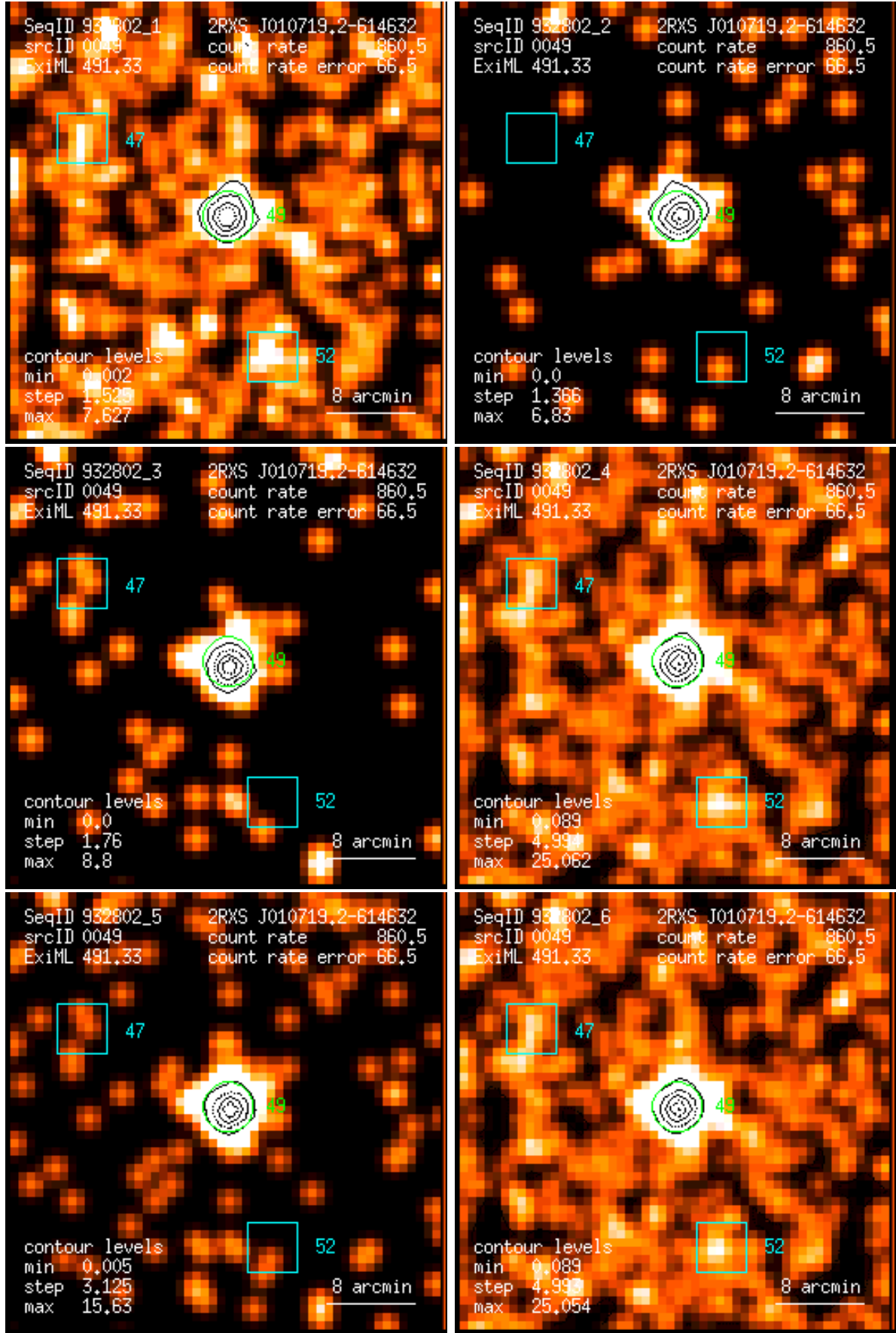
Figure 49: RASS 932802: detection 0049: band rate images, Gaussian filter: (1) PSPC channels 11 – 41, (2) 52 – 90, (3) 91 – 201, (4) 11 – 235, (5) 52 – 201, (6) 11 – 201. Broad band rates in counts/ks. Band rate contour levels in counts/ks/arcmin 2 .
