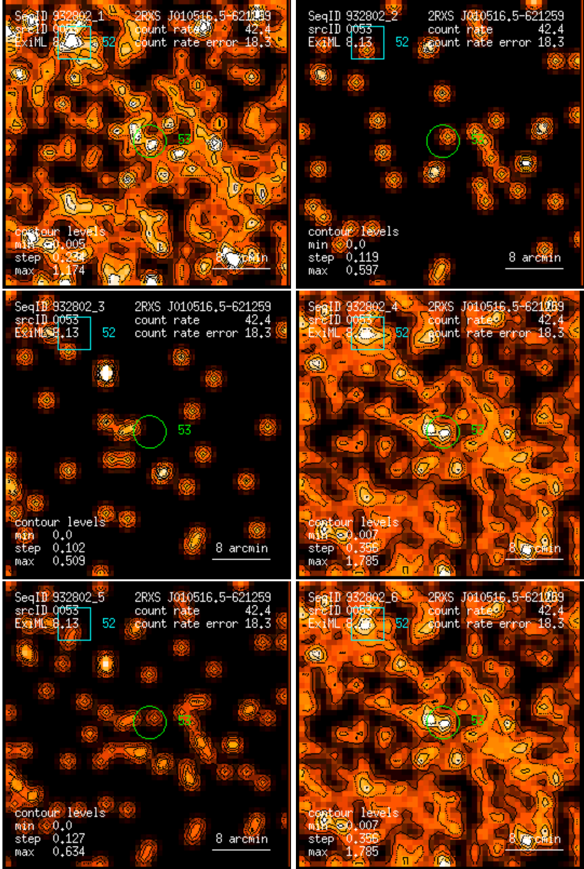
Figure 53: RASS 932802: detection 0053: band rate images, Gaussian filter: (1) PSPC channels 11 – 41, (2) 52 – 90, (3) 91 – 201, (4) 11 – 235, (5) 52 – 201, (6) 11 – 201. Broad band rates in counts/ks. Band rate contour levels in counts/ks/arcmin 2 .
