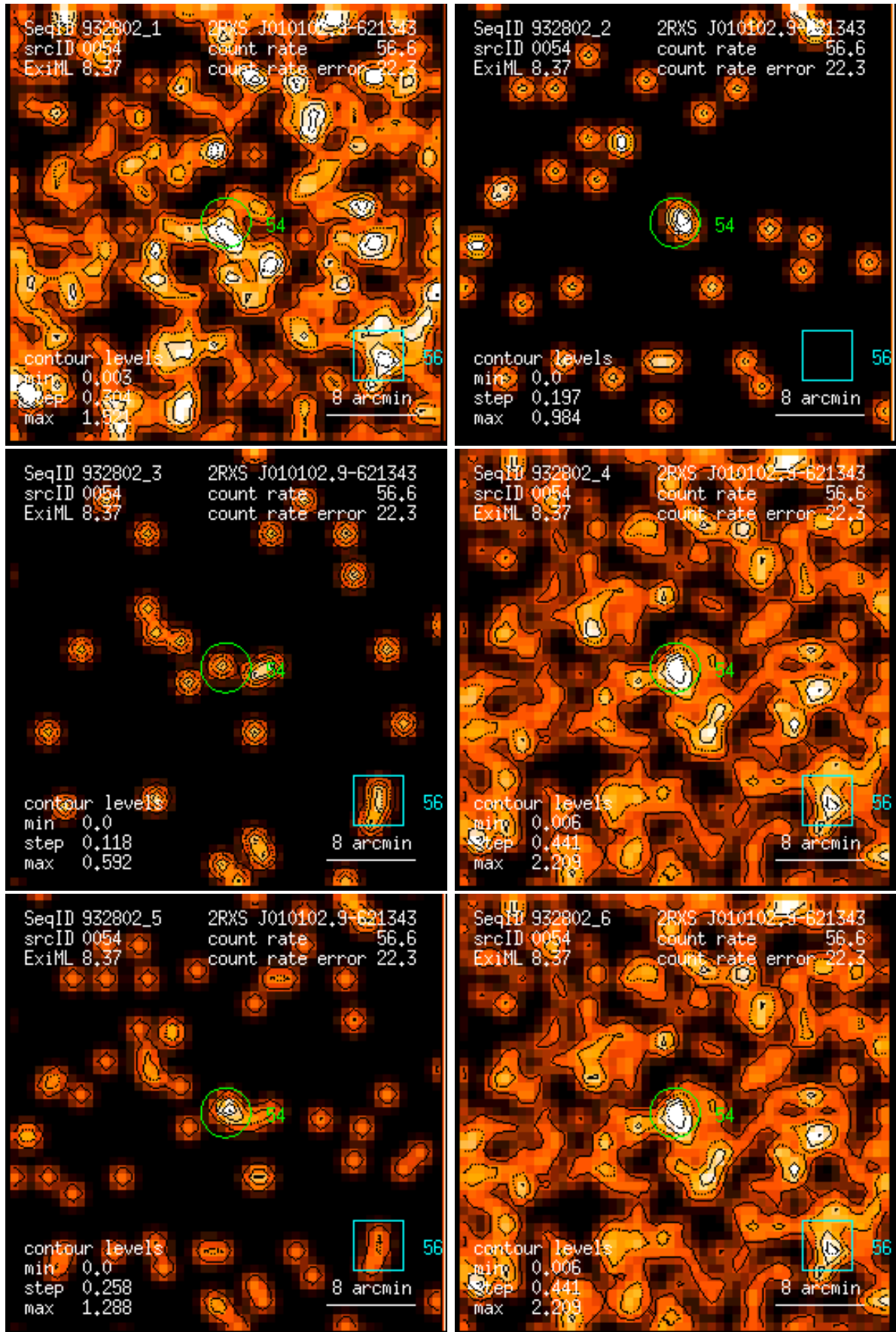
Figure 54: RASS 932802: detection 0054: band rate images, Gaussian filter: (1) PSPC channels 11 – 41, (2) 52 – 90, (3) 91 – 201, (4) 11 – 235, (5) 52 – 201, (6) 11 – 201. Broad band rates in counts/ks. Band rate contour levels in counts/ks/arcmin 2 .
