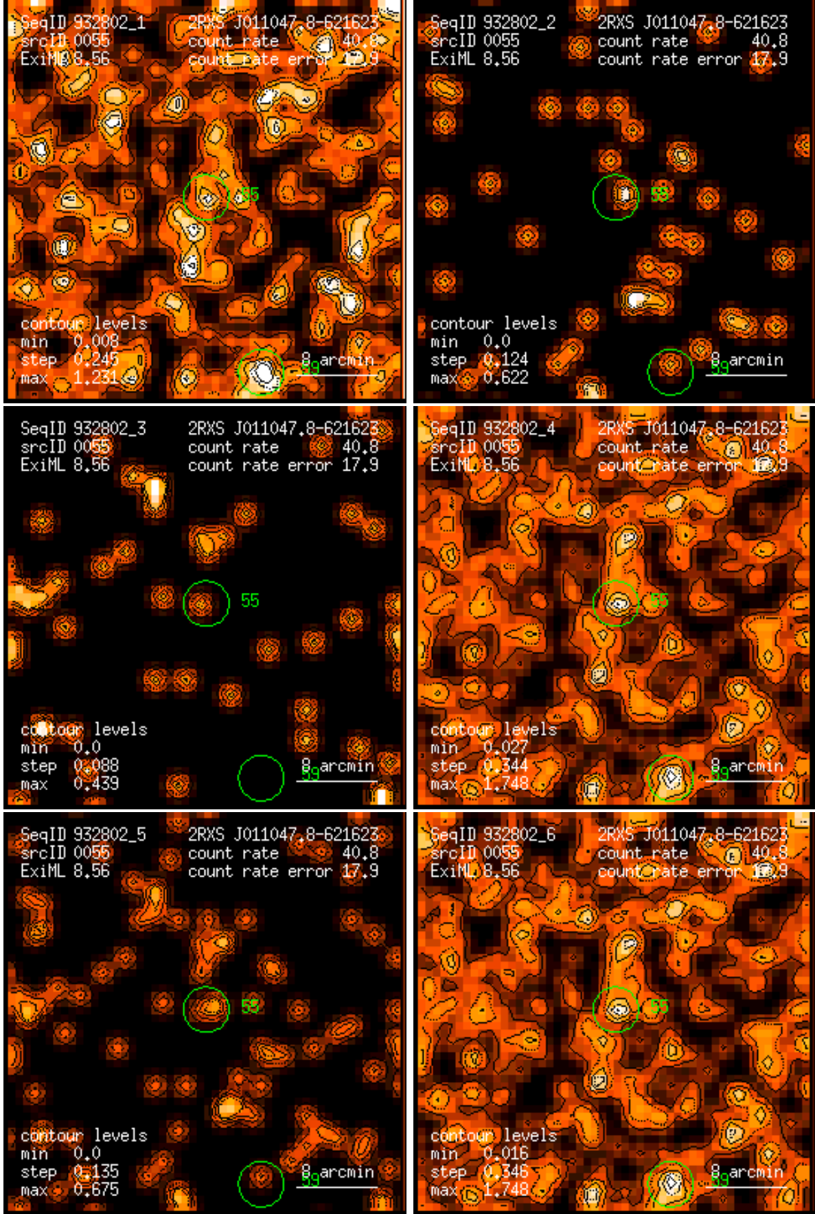
Figure 55: RASS 932802: detection 0055: band rate images, Gaussian filter: (1) PSPC channels 11 – 41, (2) 52 – 90, (3) 91 – 201, (4) 11 – 235, (5) 52 – 201, (6) 11 – 201. Broad band rates in counts/ks. Band rate contour levels in counts/ks/arcmin 2 .
