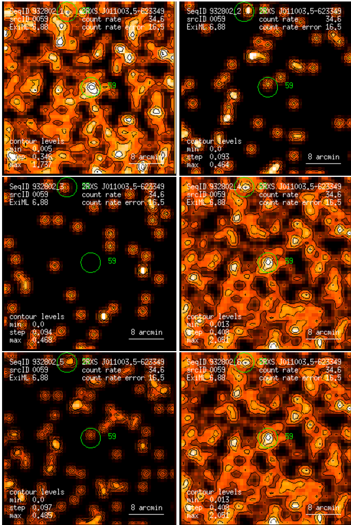
Figure 59: RASS 932802: detection 0059: band rate images, Gaussian filter: (1) PSPC channels 11 – 41, (2) 52 – 90, (3) 91 – 201, (4) 11 – 235, (5) 52 – 201, (6) 11 – 201. Broad band rates in counts/ks. Band rate contour levels in counts/ks/arcmin 2 .
