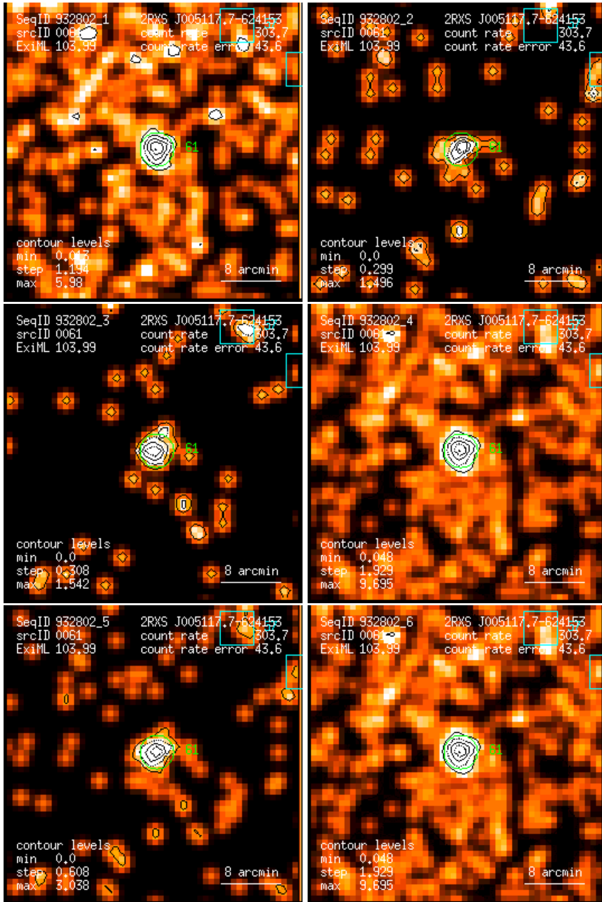
Figure 61: RASS 932802: detection 0061: band rate images, Gaussian filter: (1) PSPC channels 11 – 41, (2) 52 – 90, (3) 91 – 201, (4) 11 – 235, (5) 52 – 201, (6) 11 – 201. Broad band rates in counts/ks. Band rate contour levels in counts/ks/arcmin 2 .
